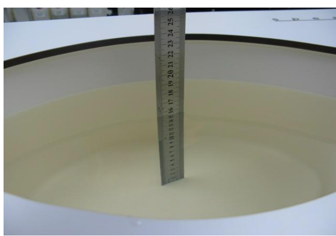
Photo 30: MSL2450MHz depth (15.1cm)
