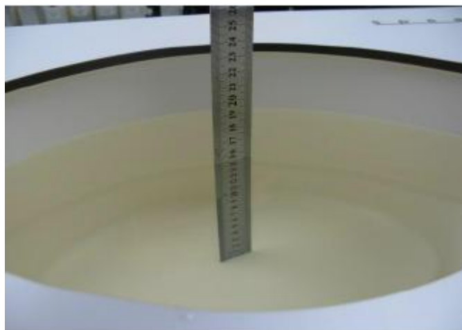
Photo 34:MBBL3500-5800MHz Depth (15.2cm)
