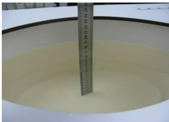
Photo 30: MSL2450MHz depth (15.1cm)
