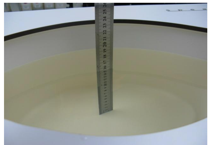
Photo 24: MSL835MHz depth (15.1cm)
