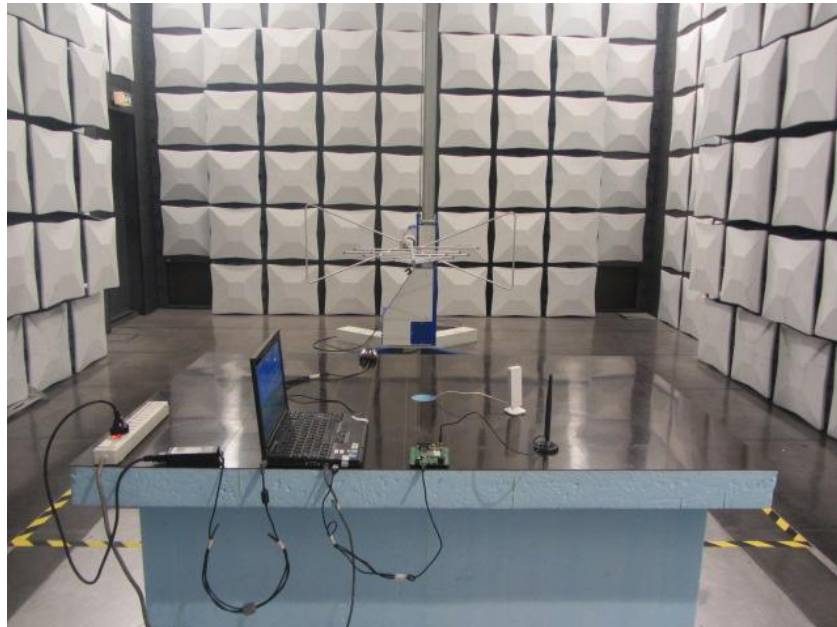
Receiver Spurious Emissions (30MHz-1GHz)
