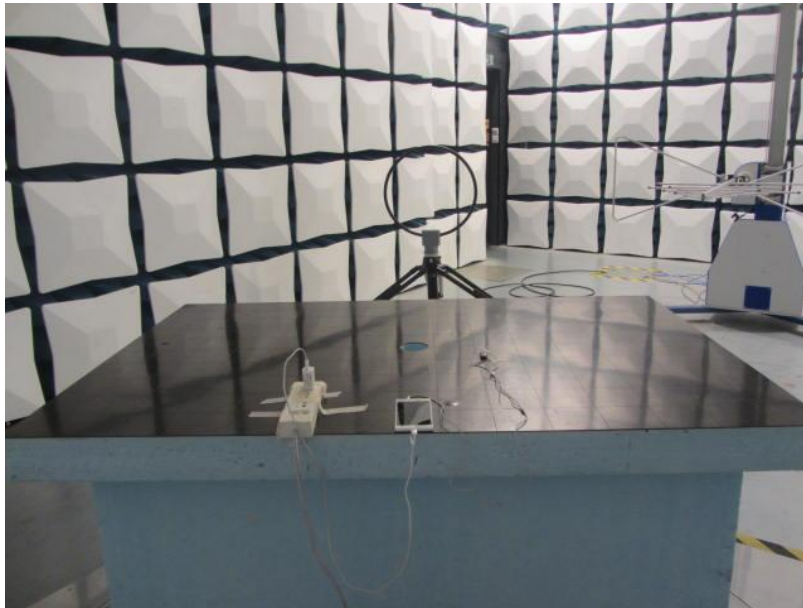
Radiated Spurious Emission (9K~30MHz)
