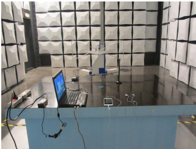
Radiated Spurious Emission (30M~1GHz)
