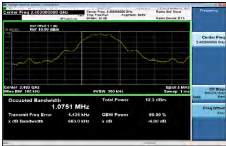
6dB Band Width Test Data CH-Low
