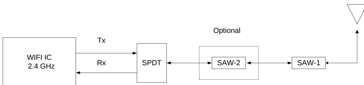
Figure 4-1 Recommended Structure
