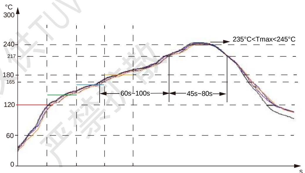
Figure 6-22 Reflow profile
