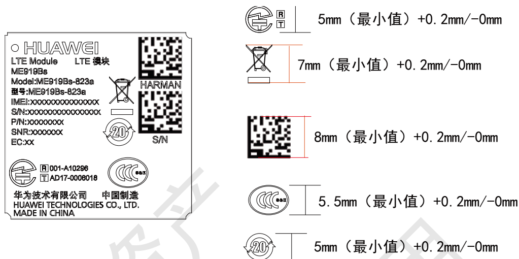
Figure 6-12 ME919Bs-823a Label
