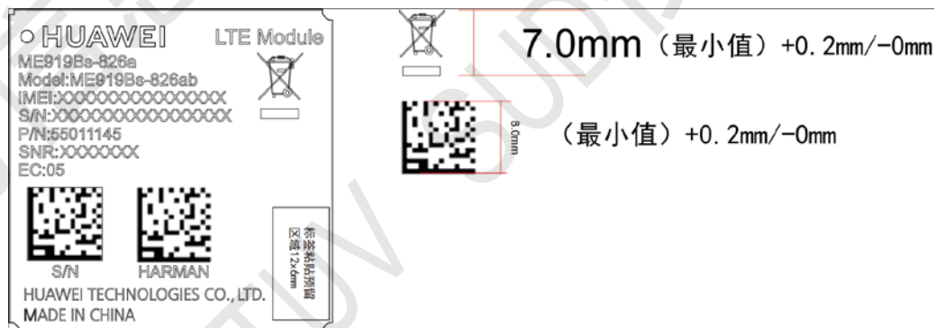
Figure 6-15 ME919Bs-826ab Label
