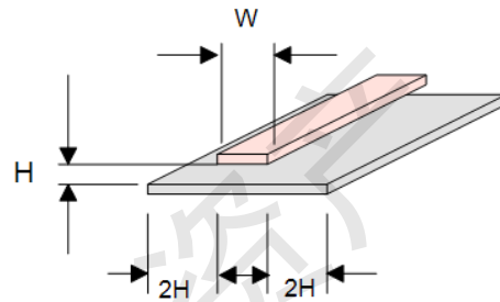
Figure 3-22 Complete structure of the microstrip
