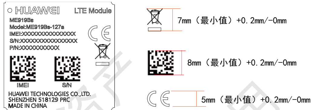
Figure 6-8 ME919Bs-127a Label
