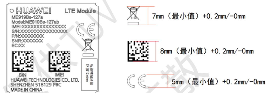
Figure 6-9 ME919Bs-127ab Label
