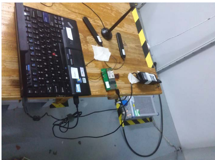
Conducted Emissions with AC Ports
