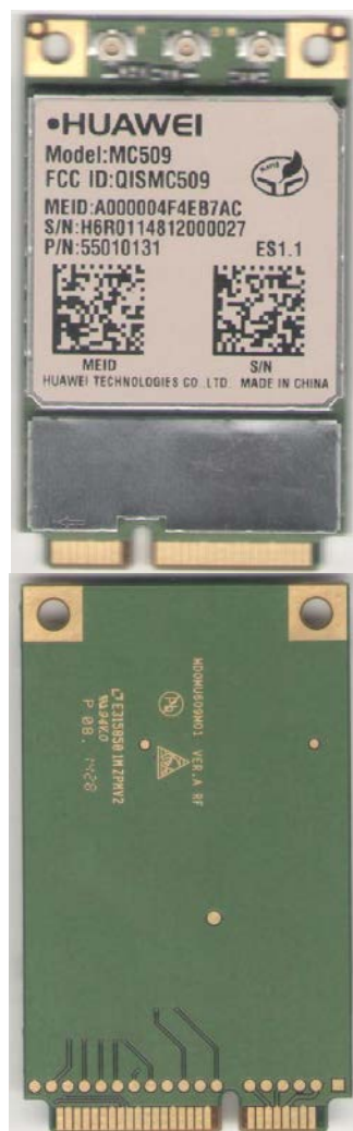
Figure1 EUT Appearance
