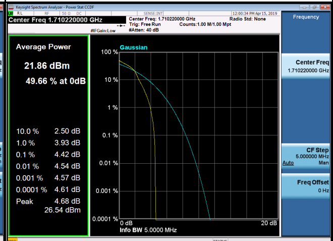
16QAM-20375
