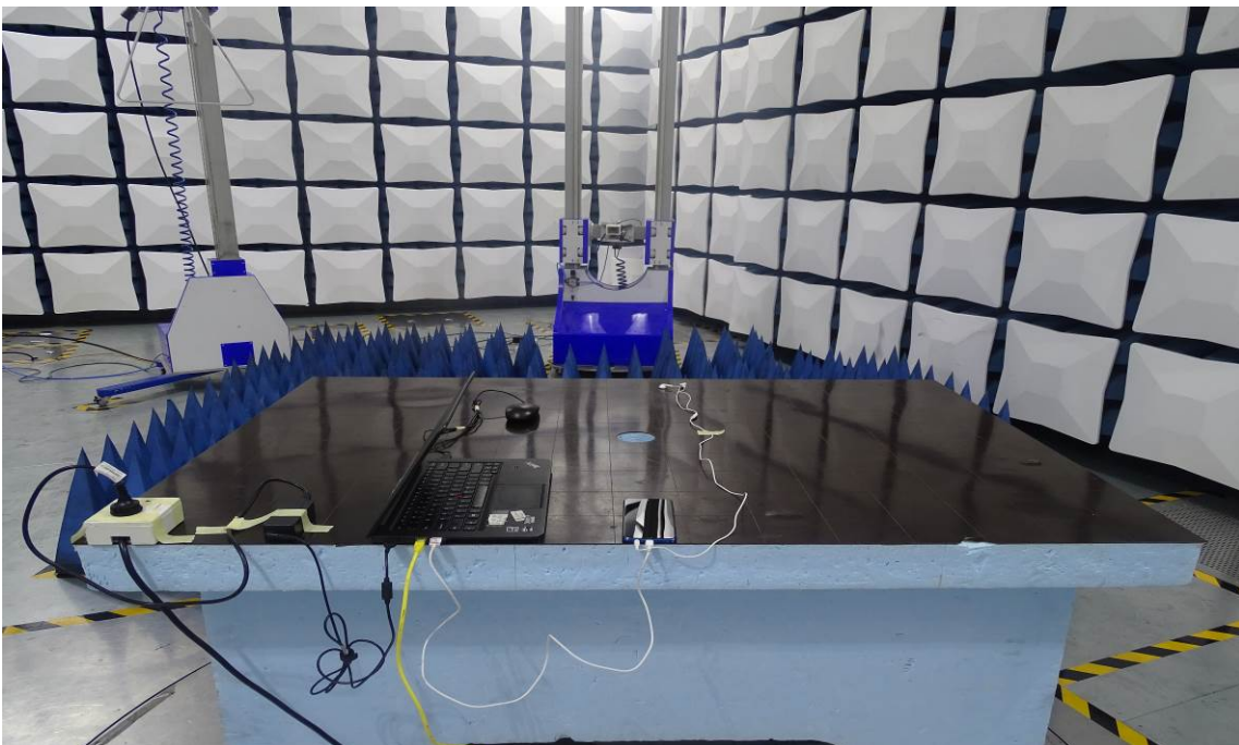
Radiated Disturbance Emissions (26.5GHz to 40GHz)
