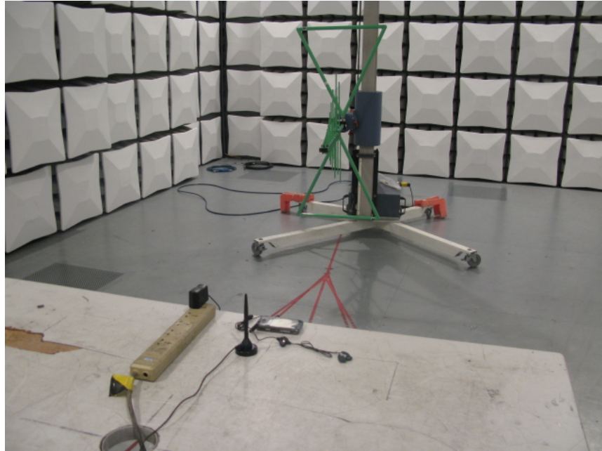
Radiated Disturbance
