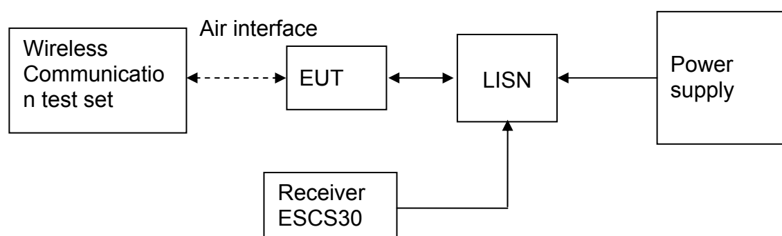
Figure 3. Test Set-up
