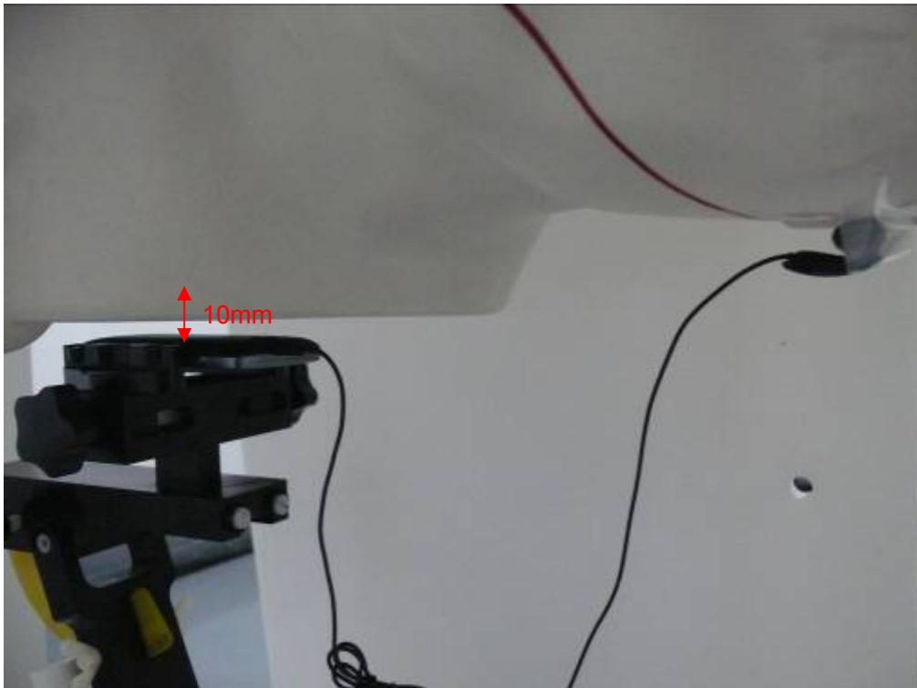
Picture 15: Body with Earphone, The EUT display towards ground, the distance from handset to the bottom of the Phantom is 10mm
