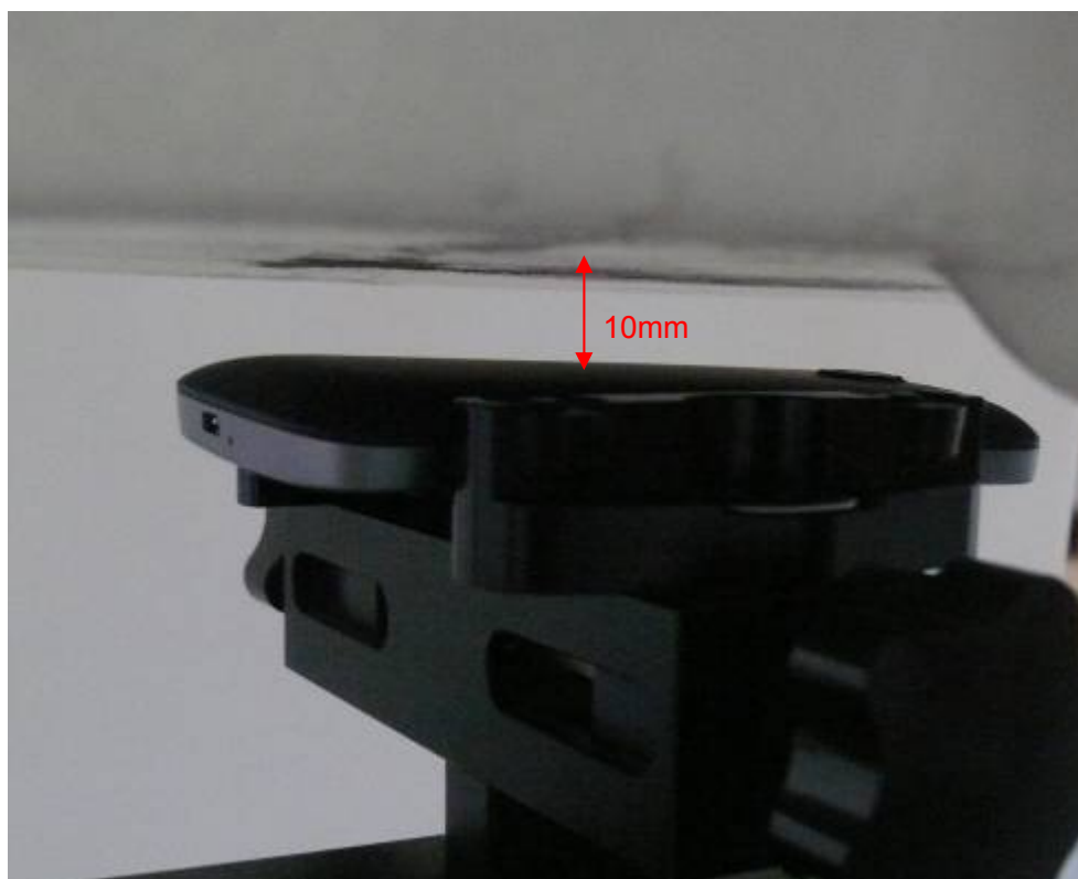
Picture 13: Body, The EUT display towards ground, the distance from handset to the bottom of the Phantom is 10mm
