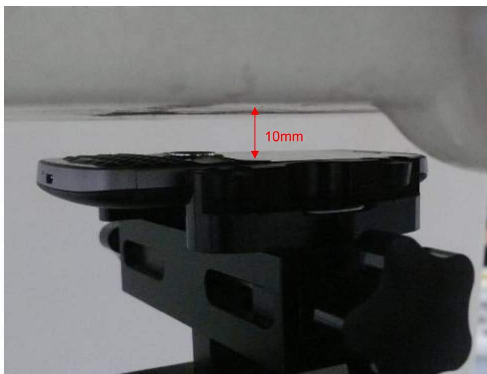
Picture 14: Body, The EUT display towards phantom, the distance from handset to the bottom of the Phantom is 10mm
