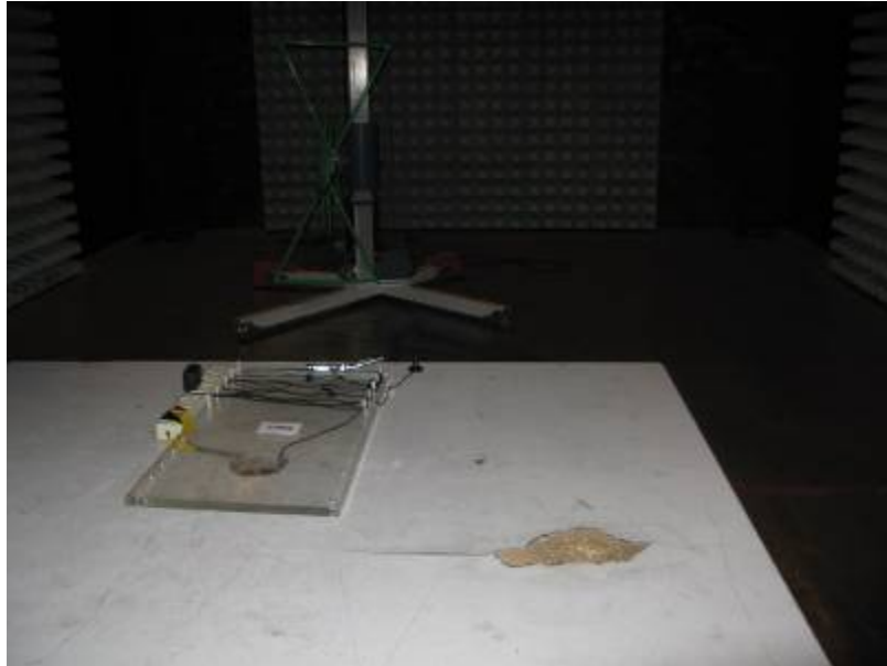
Radiated Disturbance
