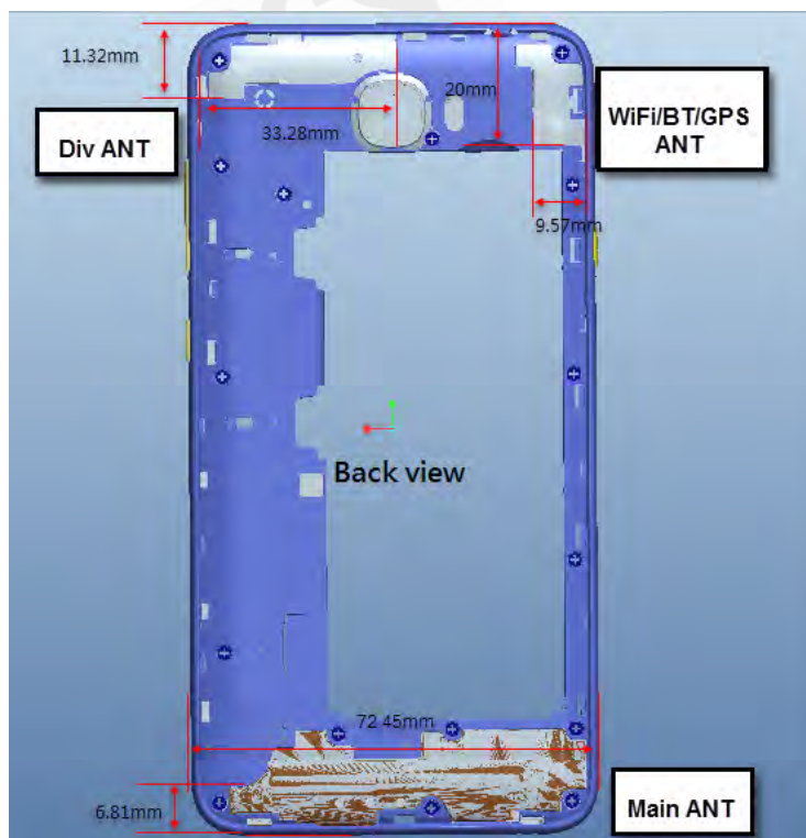
Fig.15 Antenna position of EUT
