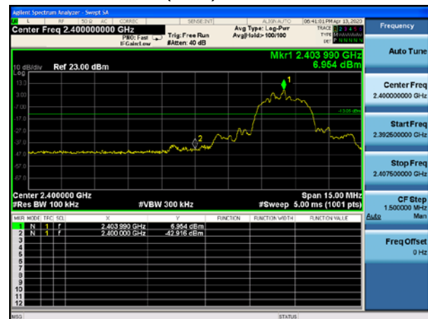
BT 4MHz \pi/4 -DQPSK(8Mbps), Carrier frequency (MHz): 2404
