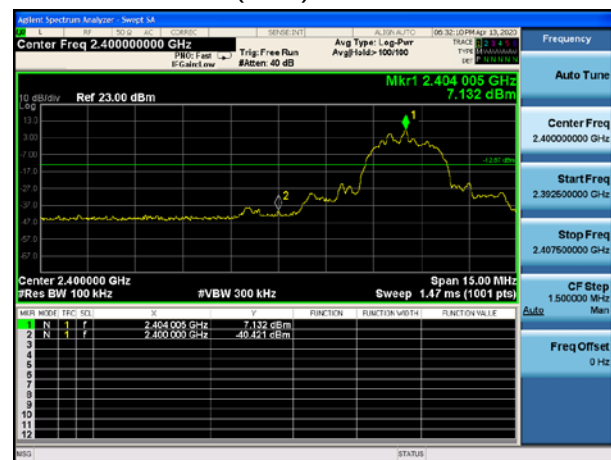
BT 2MHz 8DPSK(6Mbps), Carrier frequency (MHz): 2404
