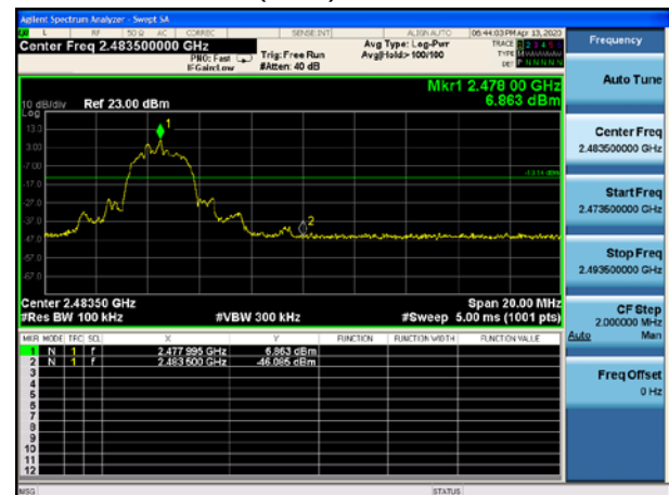
BT 4MHz \pi/4 -DQPSK(8Mbps), Carrier frequency (MHz): 2476
