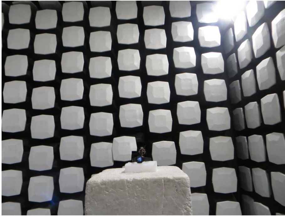
7. Radiated Emissions (Part 22/24) (Above 3GHz)
