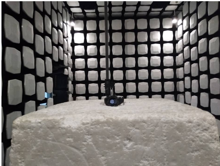
8. Radiated Emissions (Part 22/24) (Above 18GHz)
