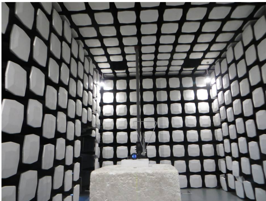
6. Radiated Emissions (Part 22/24) (below 3GHz)
