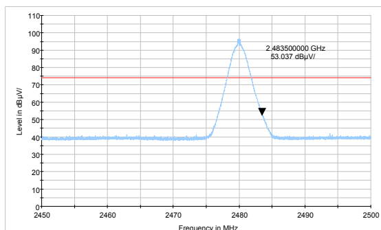
3DH5-Channel 78: Peak
