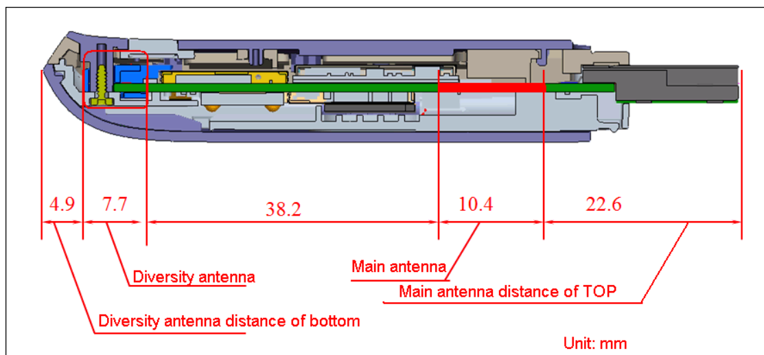
Picture 6: Antenna
