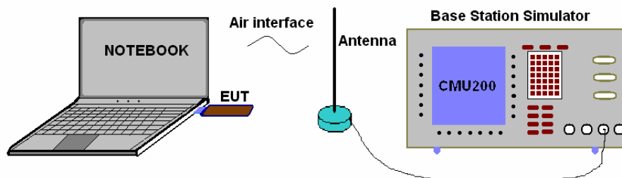
Figure 2. TC1 (TM11-TM20)
