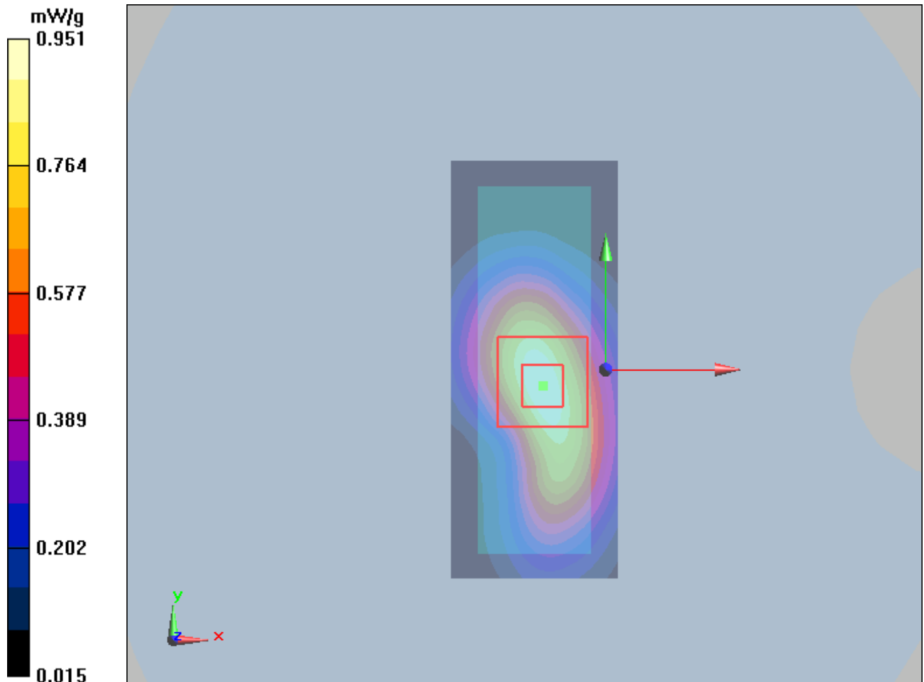
Figure 18 GSM 1900 GPRS (3TXslots) with IBM T61 Test Position 2 Channel 512
