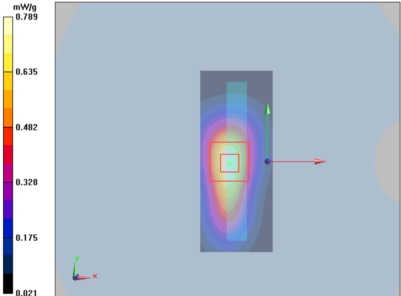
Figure 20 GSM 1900 GPRS (3TXslots) with Lenovo Y-450 Test Position 3 Channel 661
