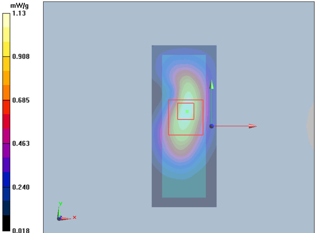
Figure 24 GSM 1900 GPRS (3TXslots) with IBM T61 Test Position 1 Channel 512
