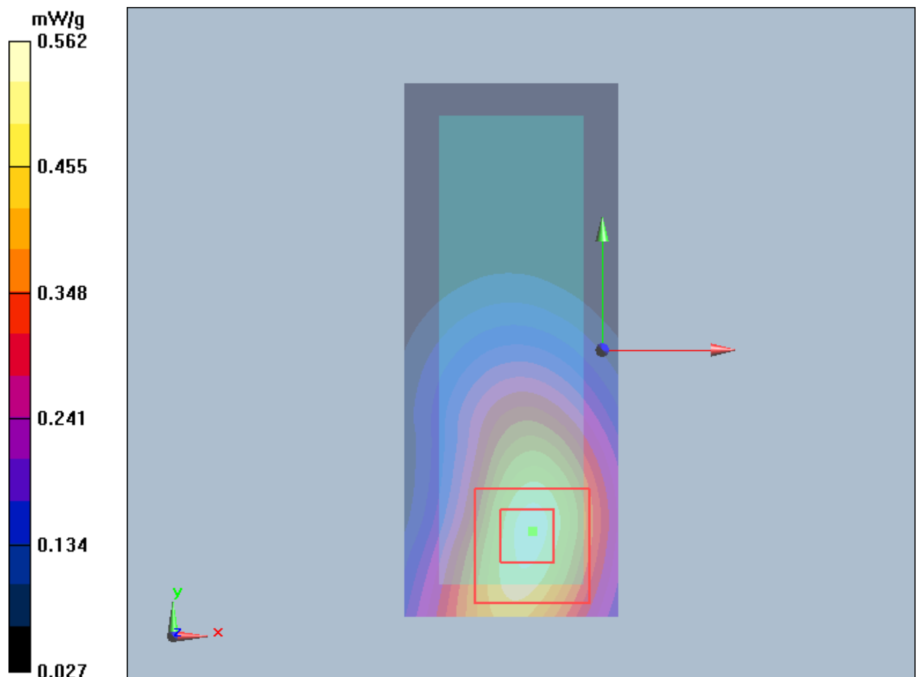
Figure 28 UMTS Band V with IBM T61 Test Position 2 Channel 4183
