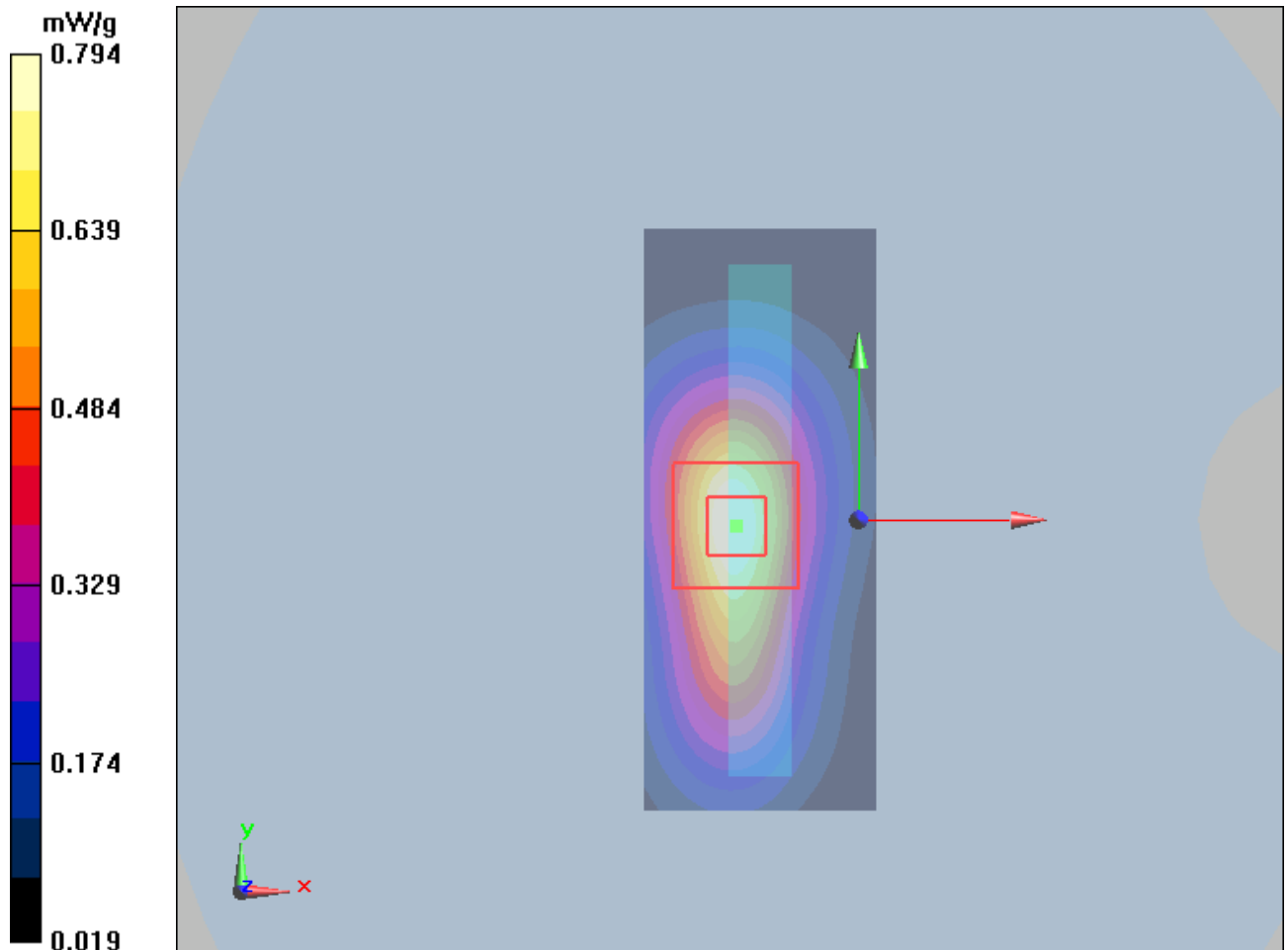
Figure 19 GSM 1900 GPRS (3TXslots) with Lenovo Y-450 Test Position 3 Channel 810
