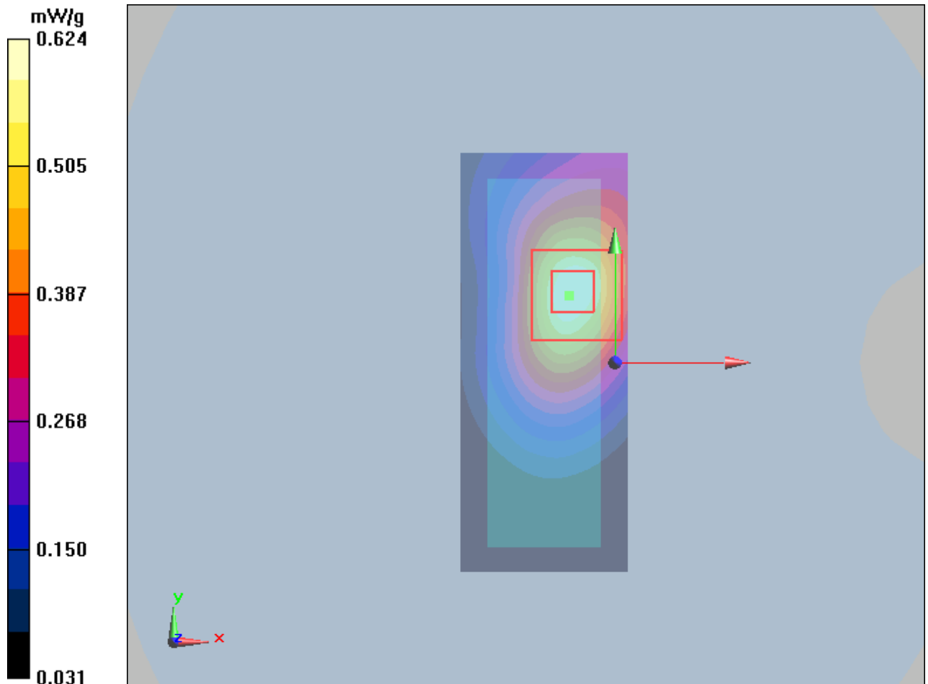
Figure 27 UMTS Band V with IBM T61 Test Position 1 Channel 4132
