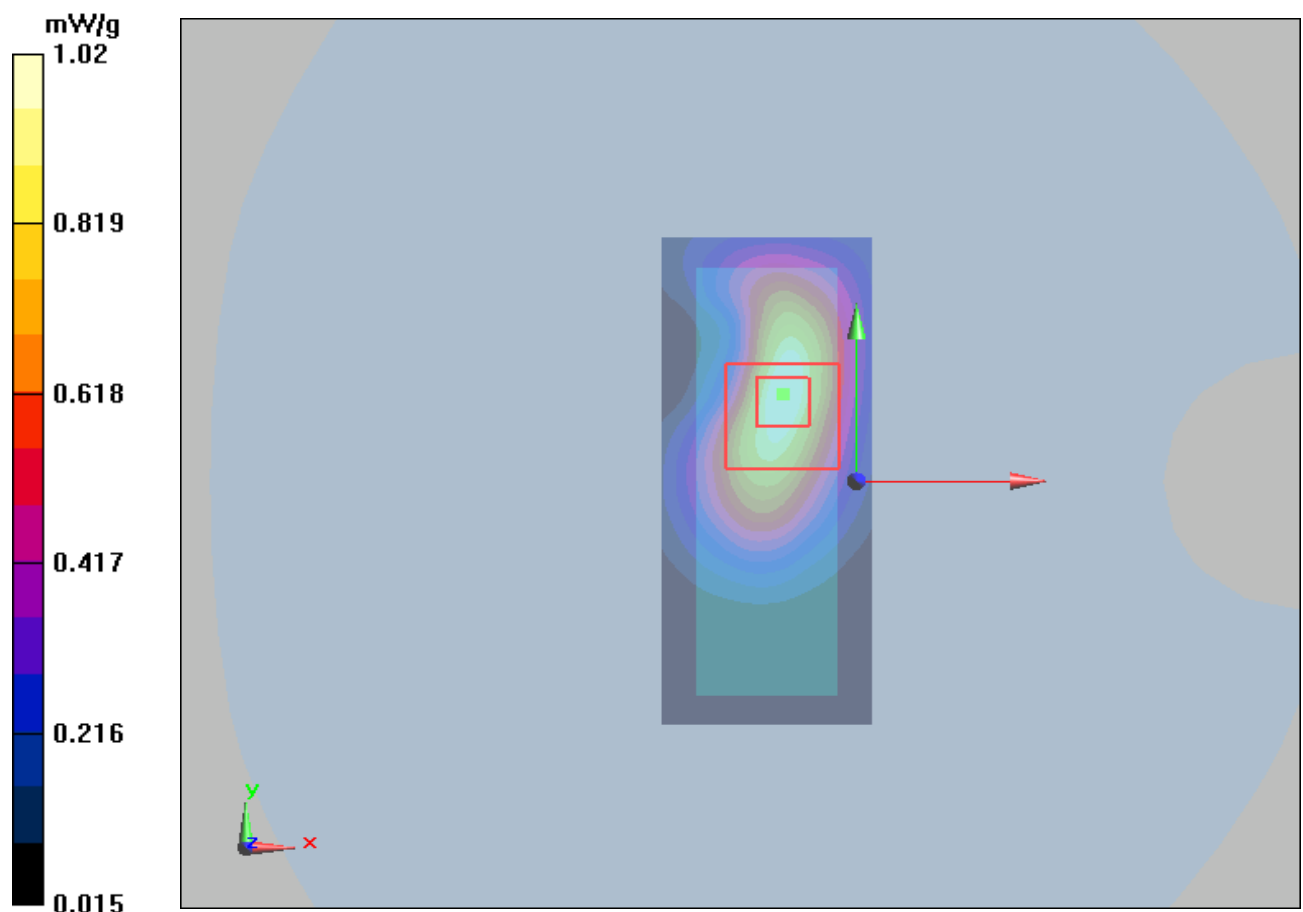
Figure 13 GSM 1900 GPRS (3TXslots) with IBM T61 Test Position 1 Channel 810
