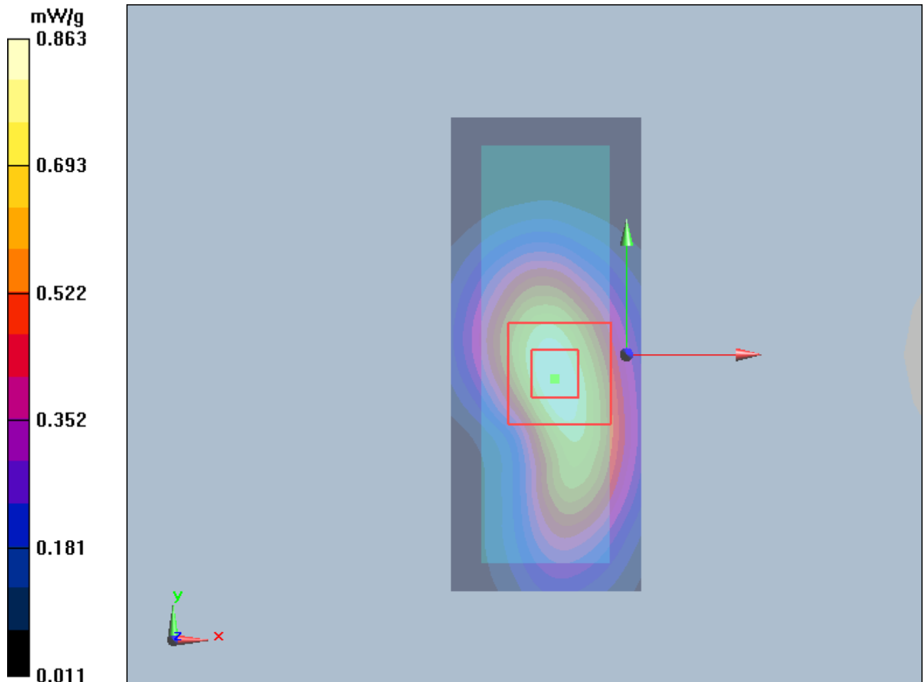
Figure 16 GSM 1900 GPRS (3TXslots) with IBM T61 Test Position 2 Channel 810
