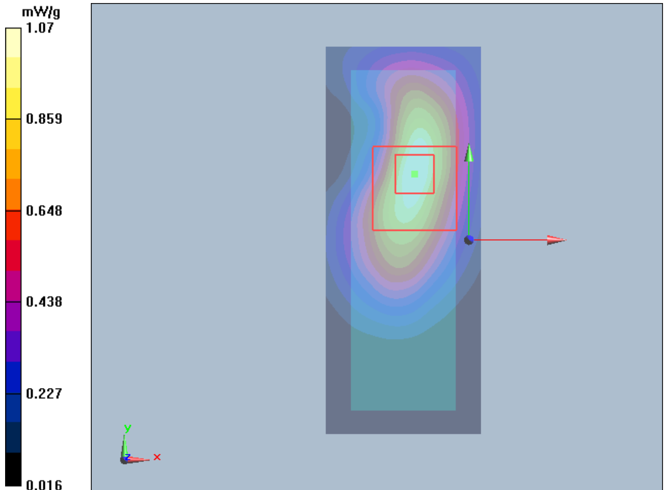
Figure 14 GSM 1900 GPRS (3TXslots) with IBM T61 Test Position 1 Channel 661
