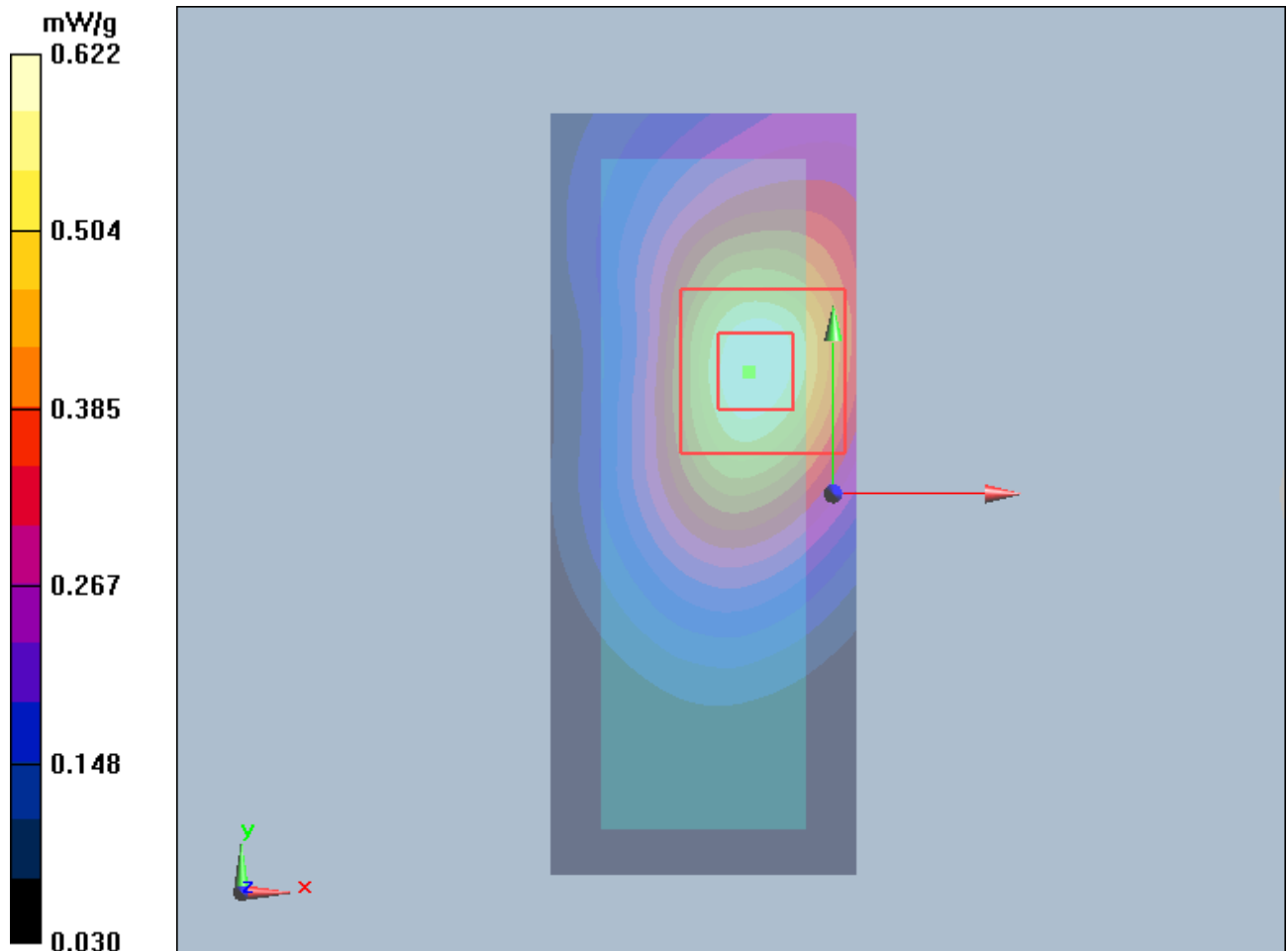
Figure 8 GSM 850 GPRS (3TXslots) with IBM T61 Test Position 1 Channel 190
