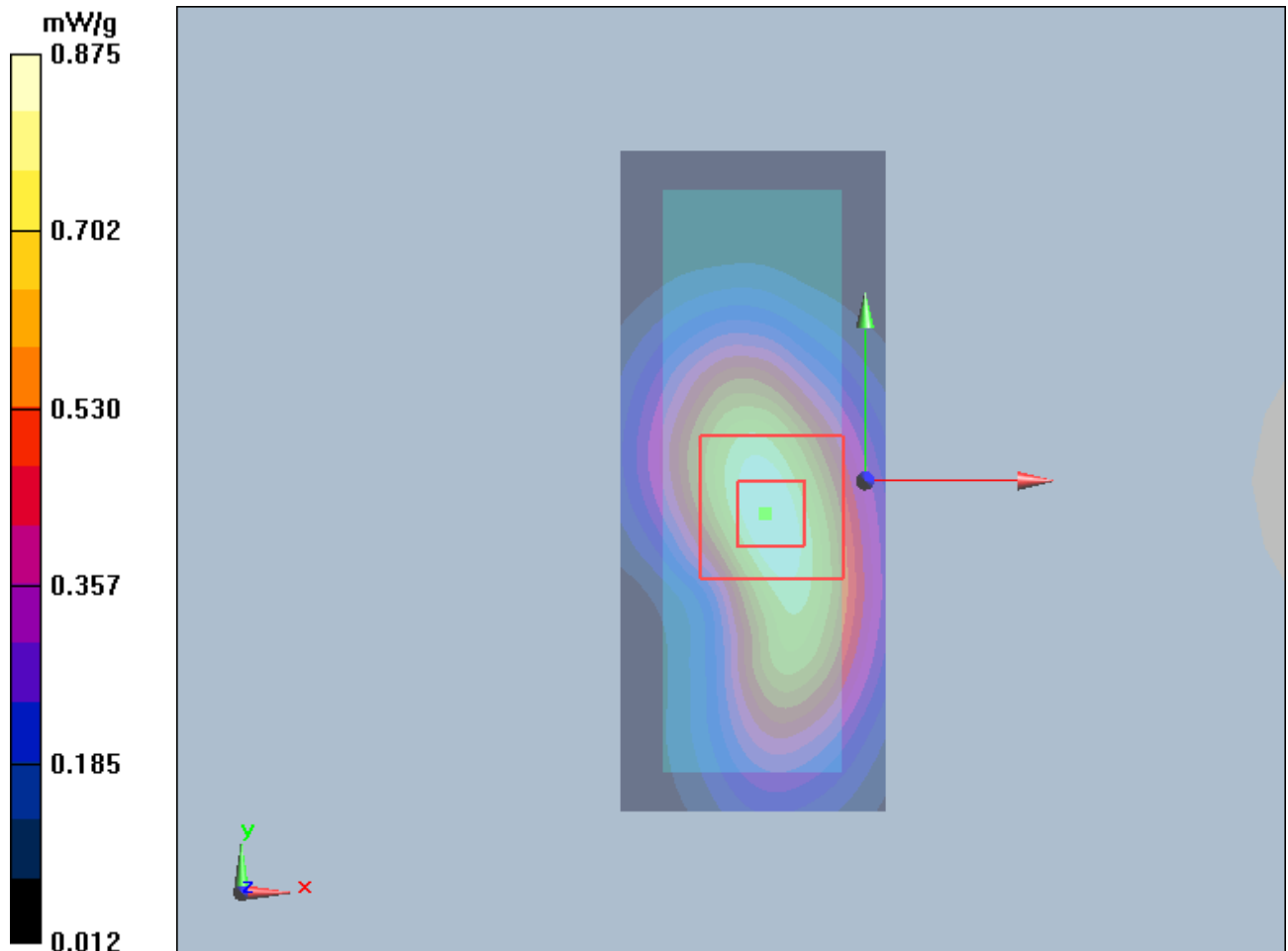
Figure 17 GSM 1900 GPRS (3TXslots) with IBM T61 Test Position 2 Channel 661
