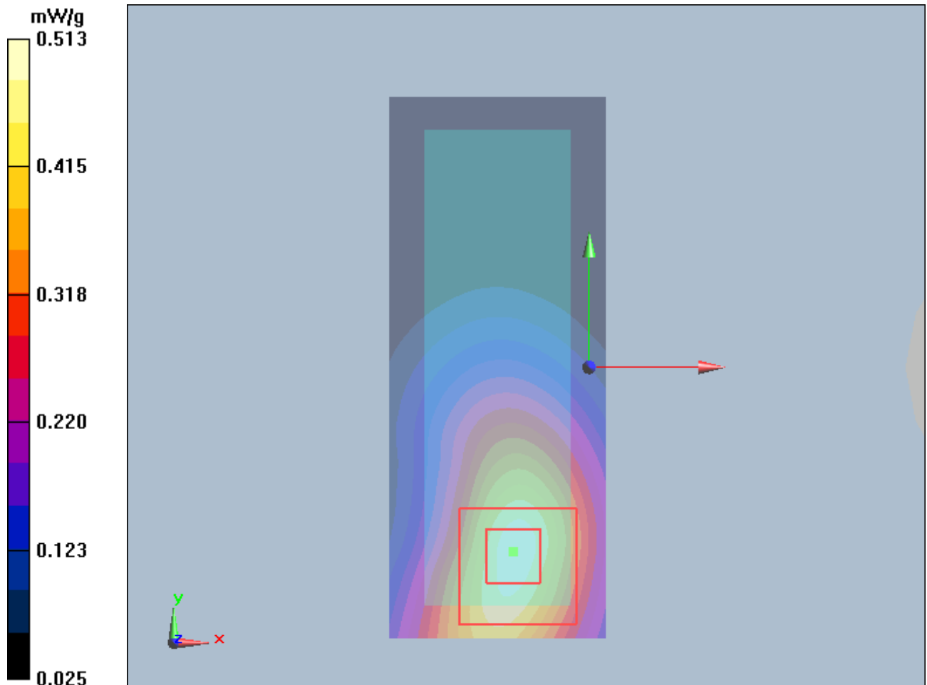
Figure 9 GSM 850 GPRS (3TXslots) with IBM T61 Test Position 2 Channel 190
