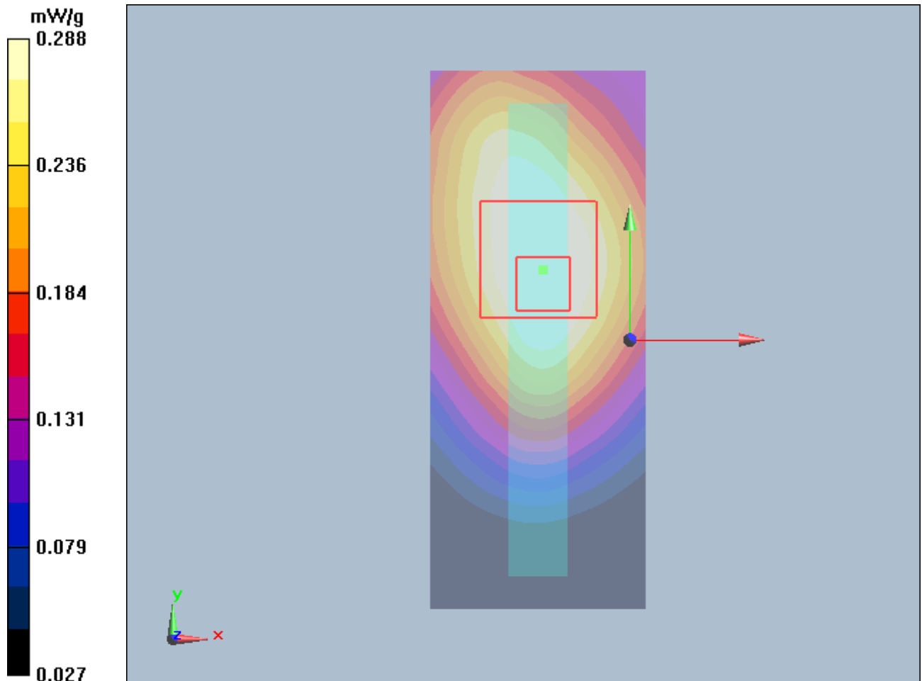
Figure 11 GSM 850 GPRS (3TXslots) with Lenovo Y-450 Test Position 4 Channel 190
