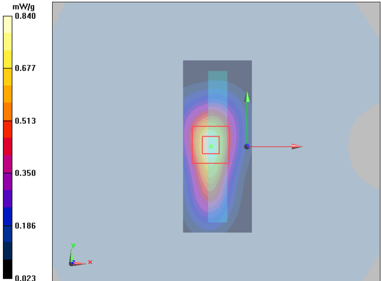
Figure 21 GSM 1900 GPRS (3TXslots) with Lenovo Y-450 Test Position 3 Channel 512
