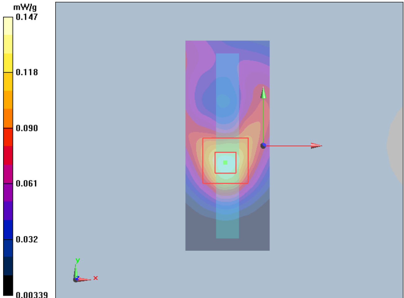
Figure 22 GSM 1900 GPRS (3TXslots) with Lenovo Y-450 Test Position 4 Channel 661
