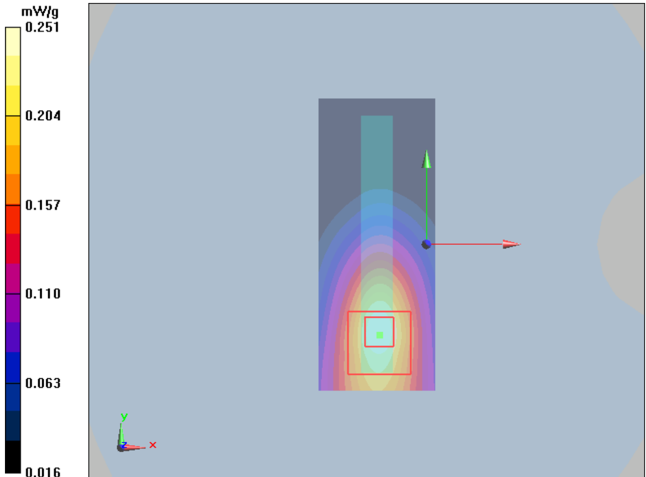
Figure 10 GSM 850 GPRS (3TXslots) with Lenovo Y-450 Test Position 3 Channel 190
