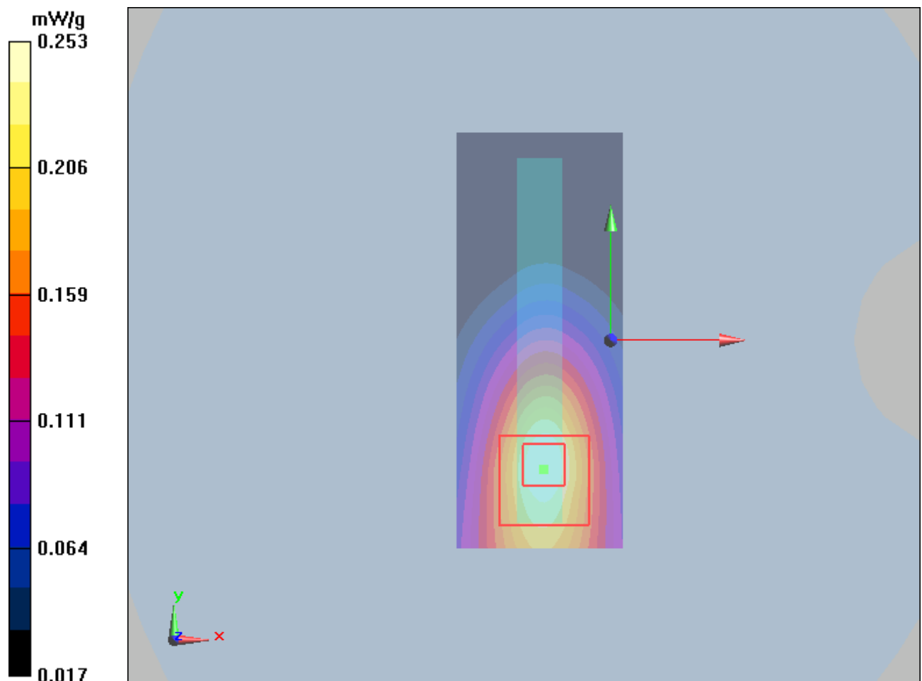
Figure 29 UMTS Band V with Lenovo Y-450 Test Position 3 Channel 4183
