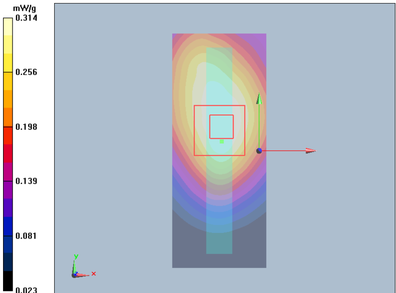
Figure 30 UMTS Band V with Lenovo Y-450 Test Position 4 Channel 4183
