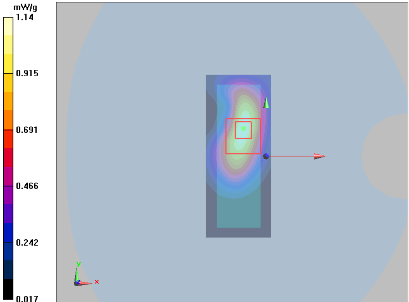
Figure 15 GSM 1900 GPRS (3TXslots) with IBM T61 Test Position 1 Channel 512
