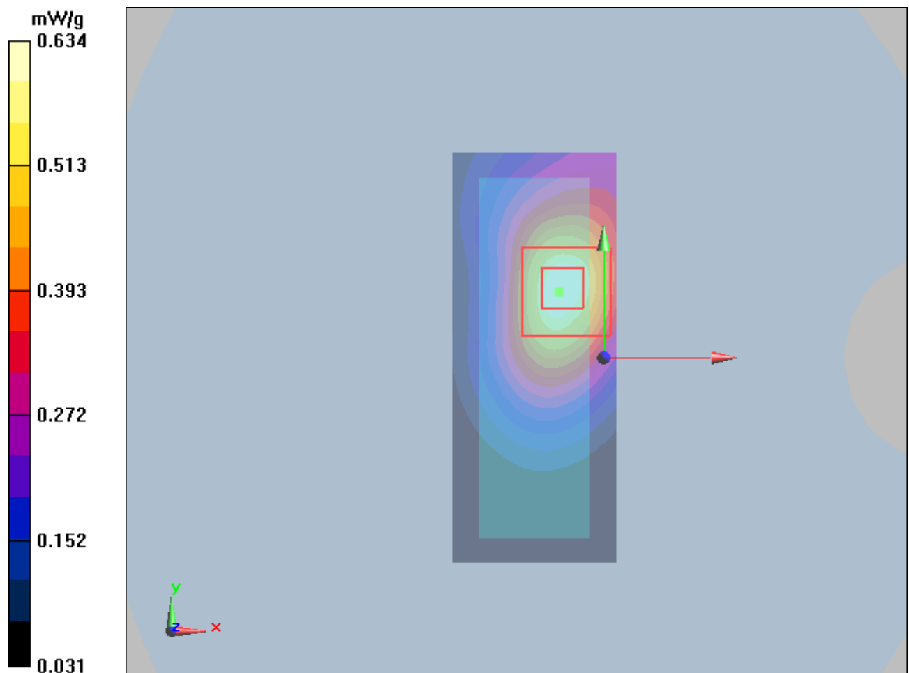
Figure 26 UMTS Band V with IBM T61 Test Position 1 Channel 4183
