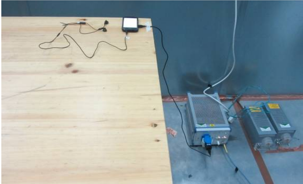
Picture 4: Conducted Emission Test Setup
