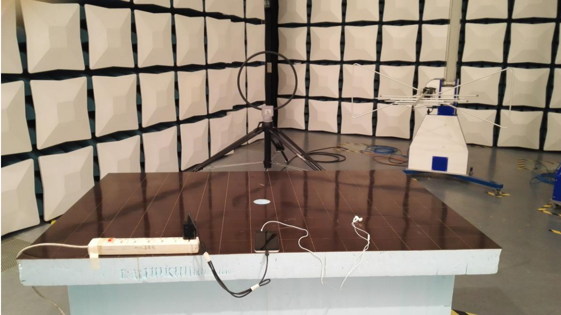
Radiated Spurious Emission (below 30MHz)
