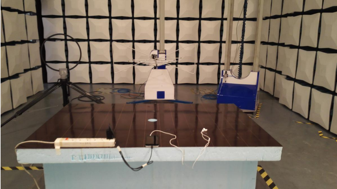
Radiated Spurious Emission (1GHz )
