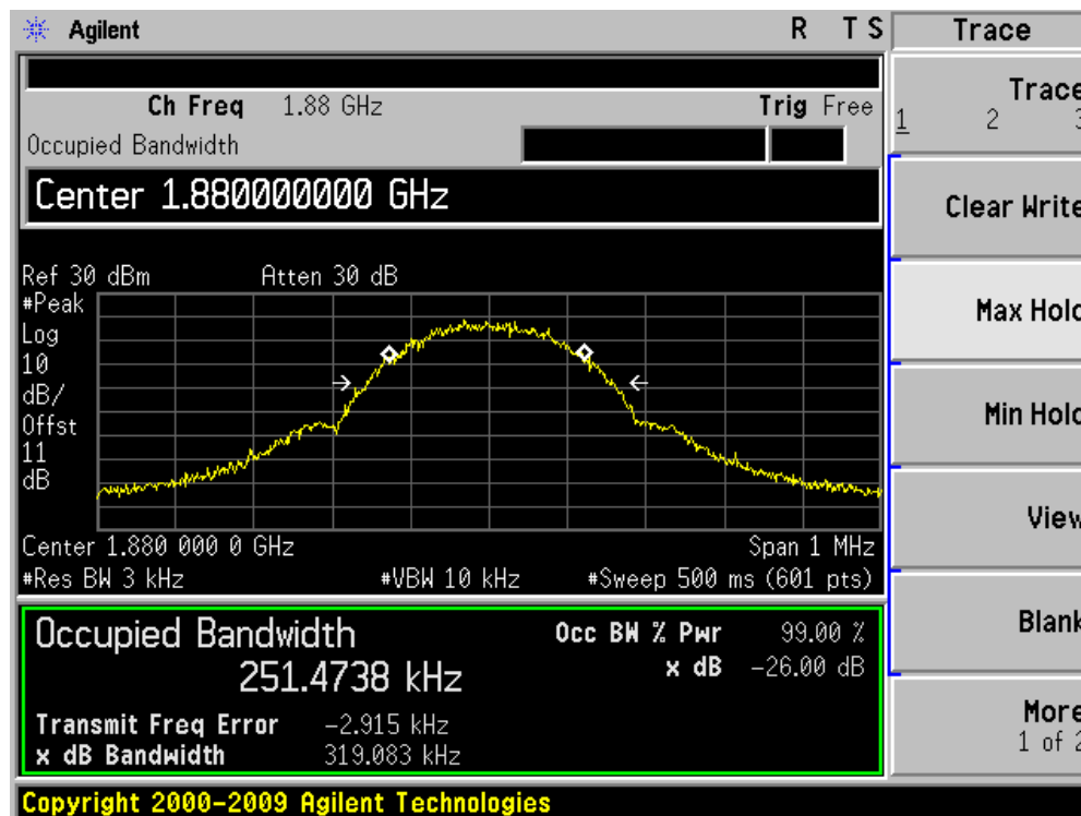
Figure Channel 661 (1880.0MHz)
