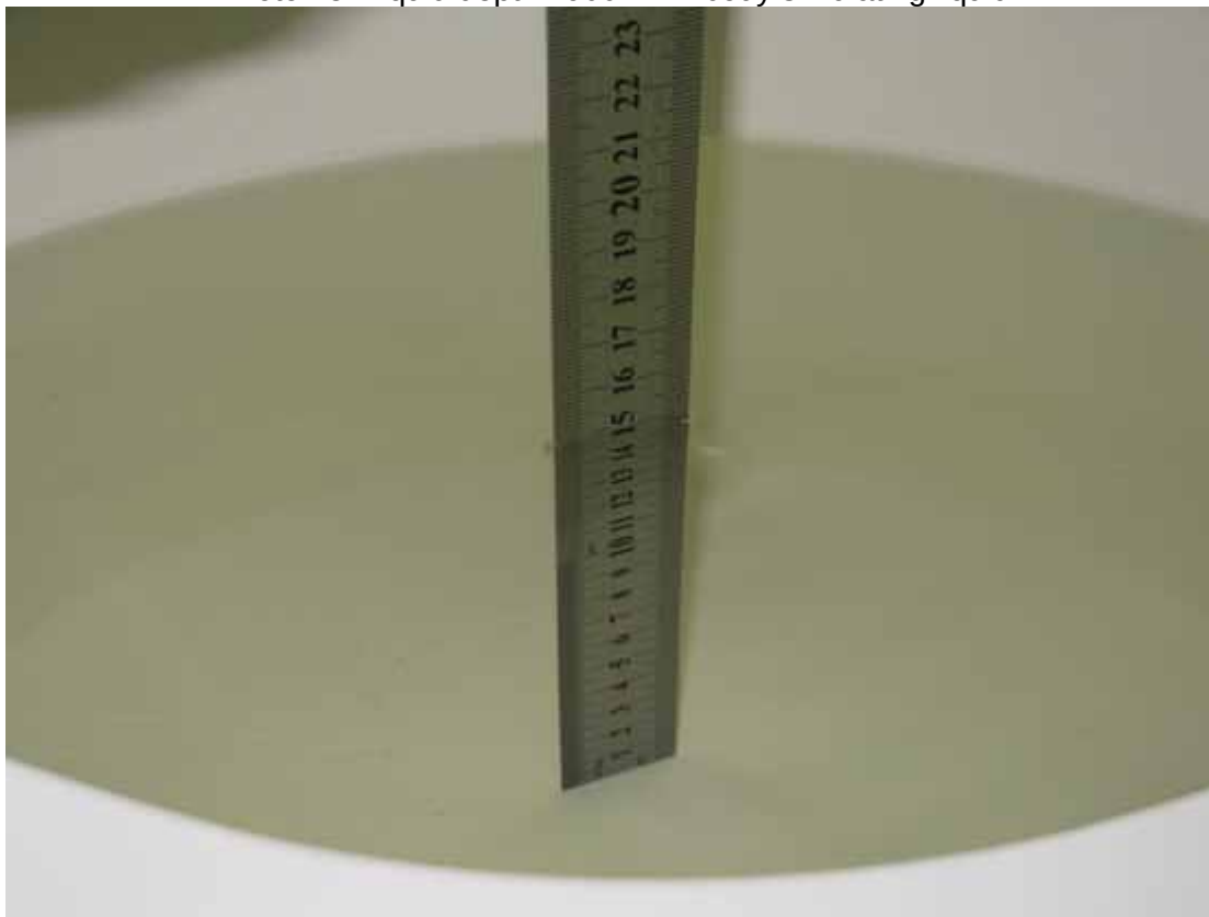
Photo 16: Liquid depth 835 MHz body simulating liquid
