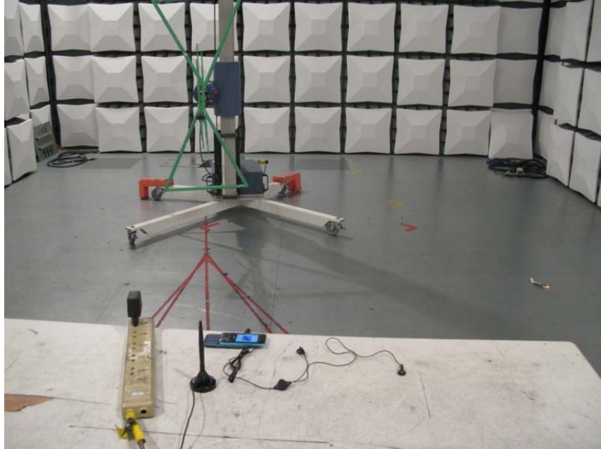
Radiated Disturbance
