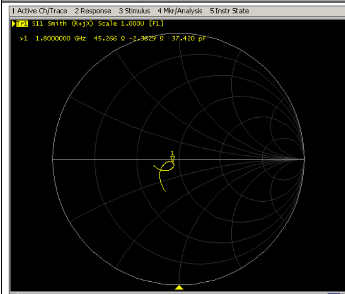
Impedance Test-Body
