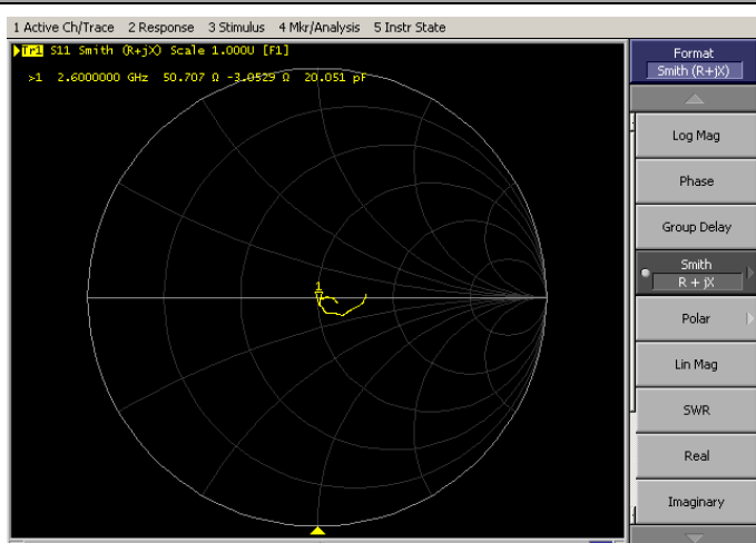
Impedance Test-Body
