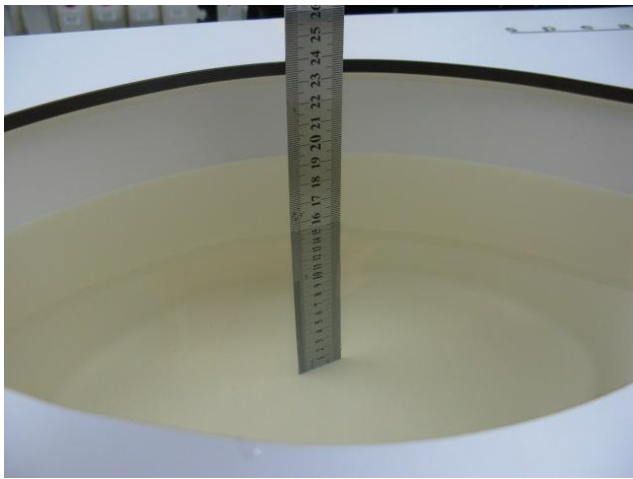
Photo 19: MSL1800MHz depth (15.1cm)
