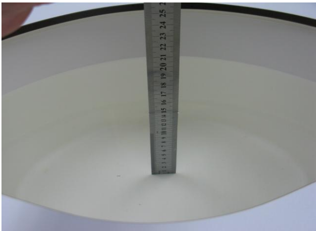
Photo 23: MSL2450MHz depth (15.1cm)
