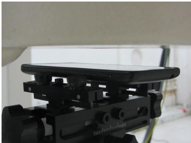
Photo 10: Towards Phantom (10mm)
