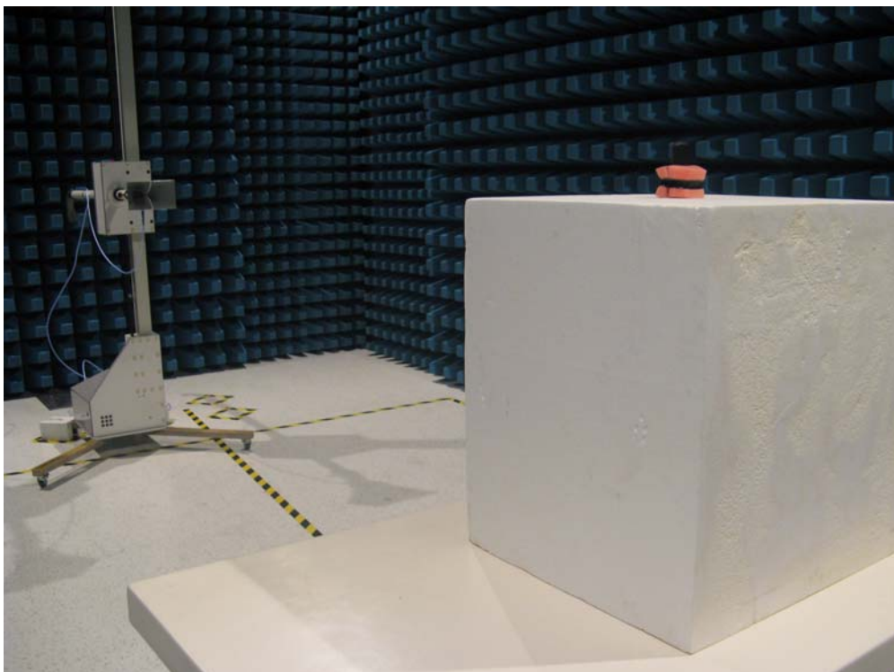
Description: PCS1900 EIRP Test Setup
