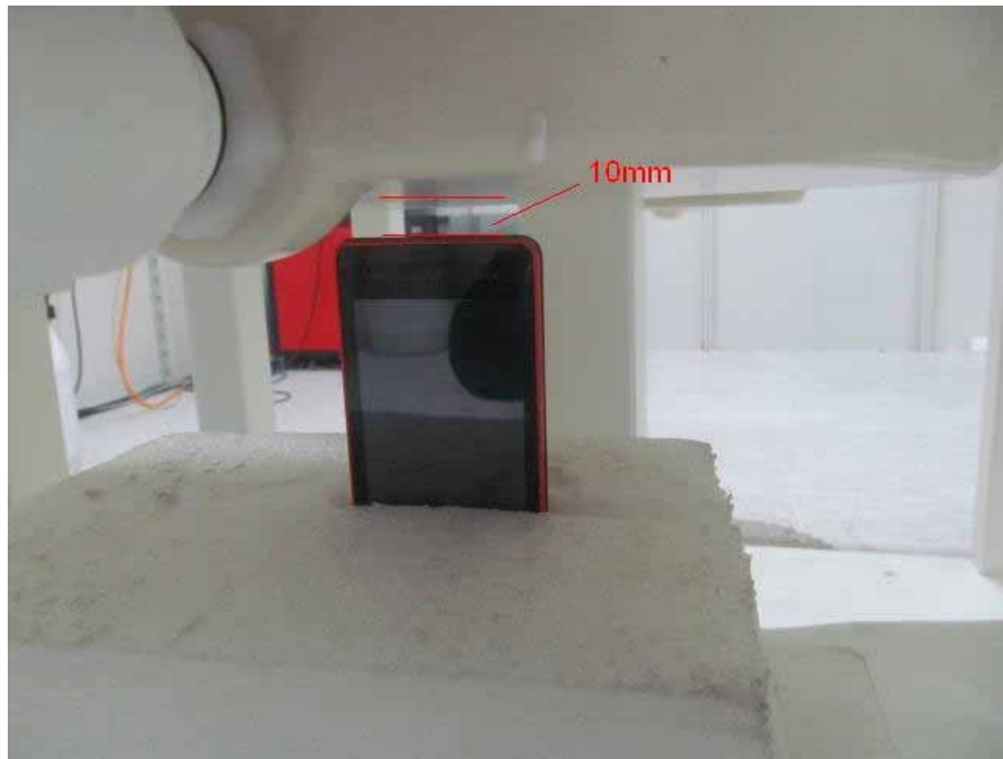
Body SAR Bottom 10mm for GSM
