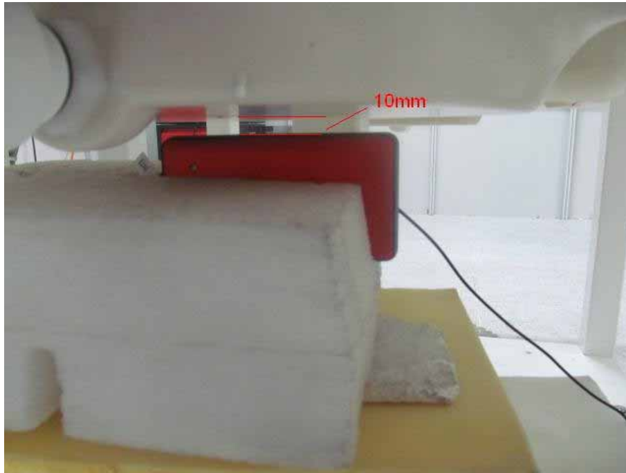
Body SAR Left Side with headset#2 10mm for GSM
