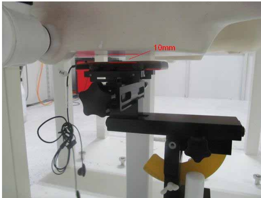
Body SAR Back 10mm with Headset#1
