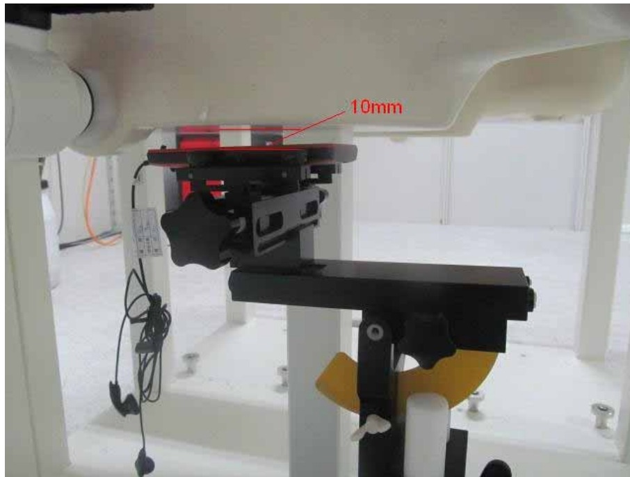
Body SAR Front 10mm with Headset#1
