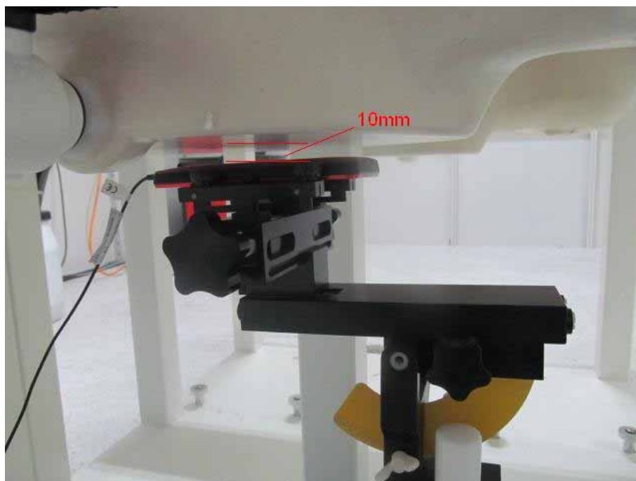
Body SAR Back 10mm with Headset#2
