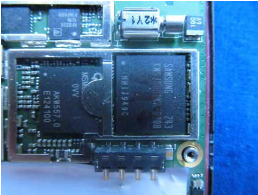
(11) EUT Photo (Single SIM Slot)
