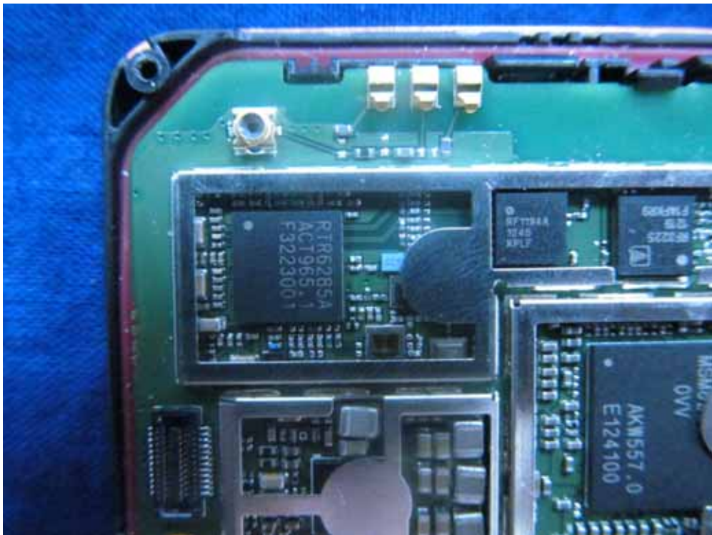
(19) EUT Photo (Dual SIM Slot)
