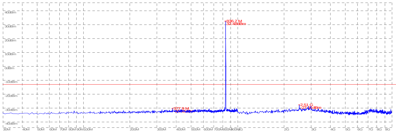
(Plot B: GSM 850MHz Channel = 190, 30MHz to 10GHz)
