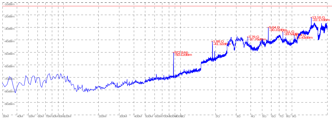
(Plot E.2: GSM 1900MHz Channel = 661, Test Antenna Vertical)
