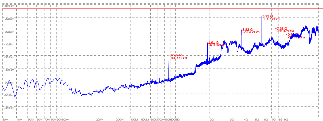
(Plot F.2: GSM 1900MHz Channel = 810, Test Antenna Vertical)
