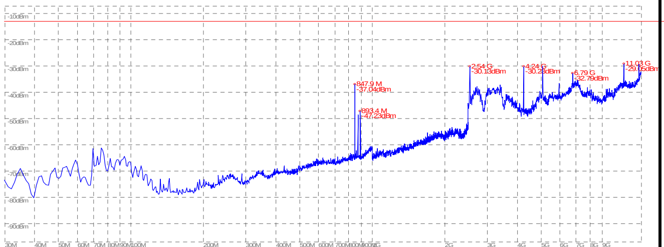
(Plot C.2: GSM 850MHz Channel = 251, Test Antenna Vertical)
