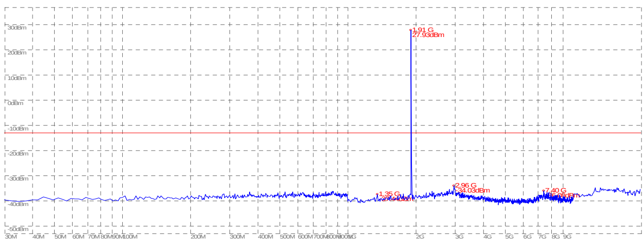
(Plot F: GSM 1900MHz Channel = 810, 30MHz to 20GHz)
