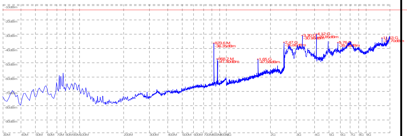
(Plot A.2: GSM 850MHz Channel = 128, Test Antenna Vertical)
