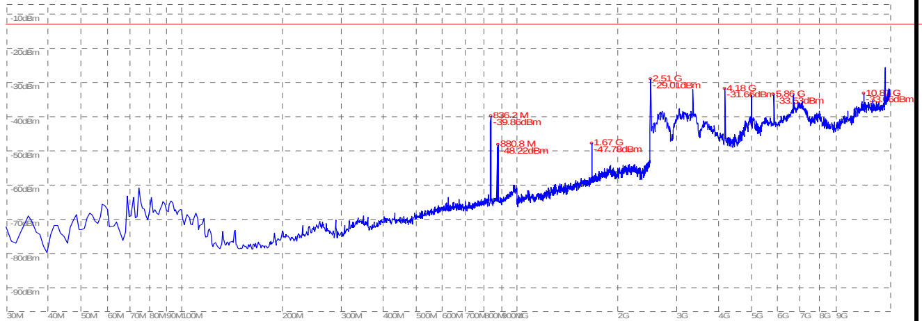
(Plot B.2: GSM 850MHz Channel = 190, Test Antenna Vertical)
