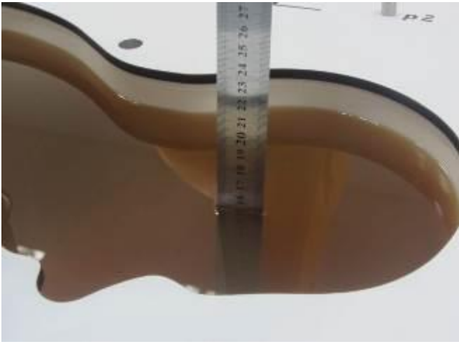
Photo 16: HBBL600-6000MHz Depth (15.1cm)
