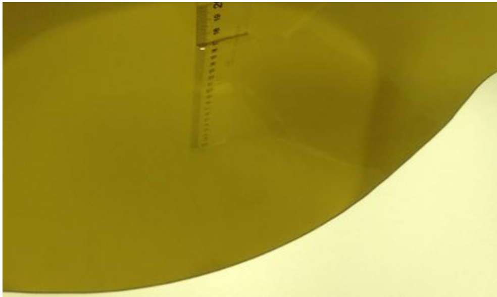
Picture 7.1: Liquid depth in the Head Phantom (835 MHz)
