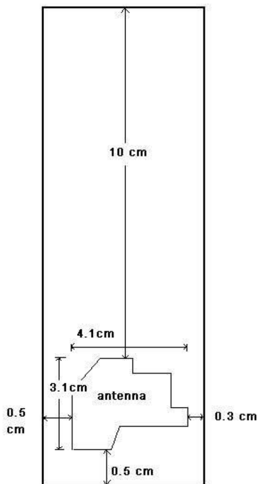
the mobile phone back antenna diagram
