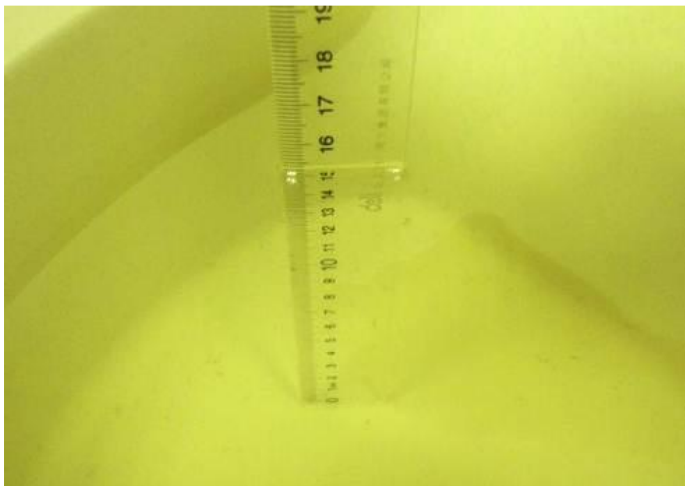
Picture 7.4 Liquid depth in the Flat Phantom (1900MHz)
