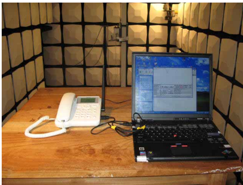
Radiated Spurious Emission (18GHz~ 26.5GHz) (TC2)
