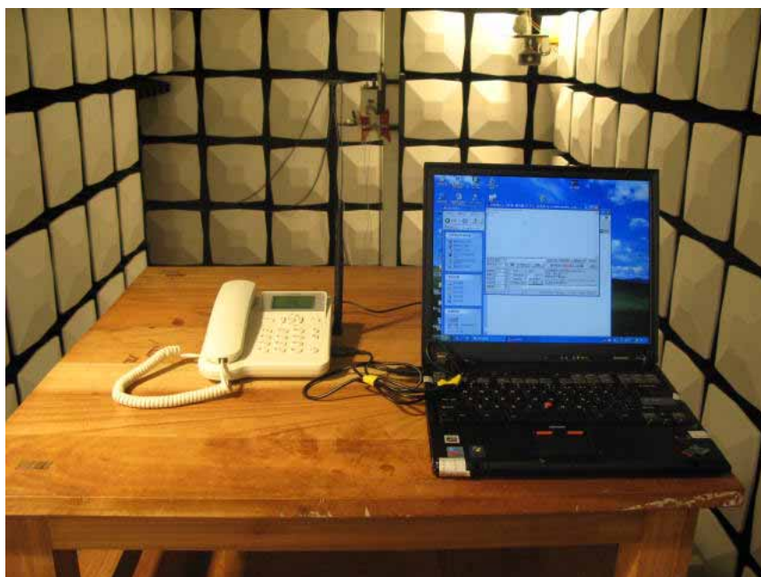
Radiated Spurious Emission (2GHz~18GHz) (TC2)
