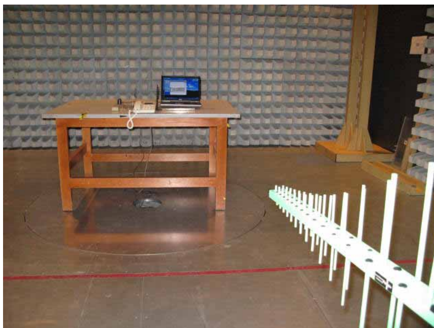
Radiated Disturbance (TC2)
