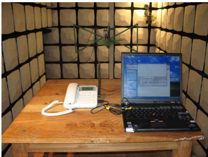
Radiated Spurious Emission (below 2GHz) (TC2)
