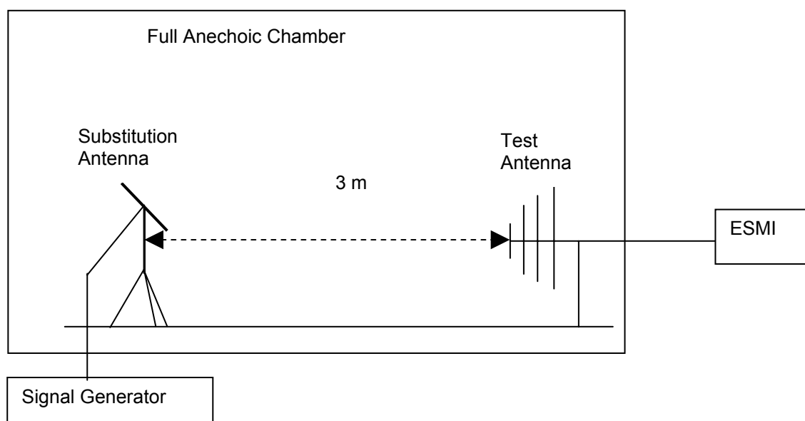
Figure 6. Test Set-up
