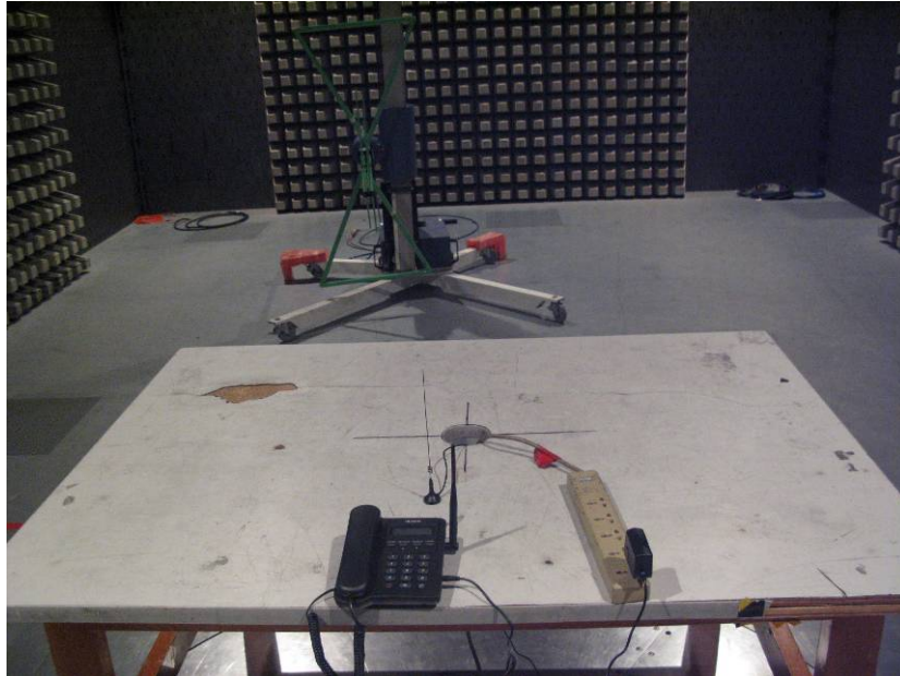
Radiated Disturbance
