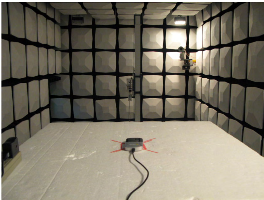
Radiated Spurious Emission (18G~26.5GHz ) CDMA
