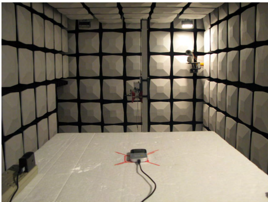
Radiated Spurious Emission (2GHz to18GHz) CDMA
