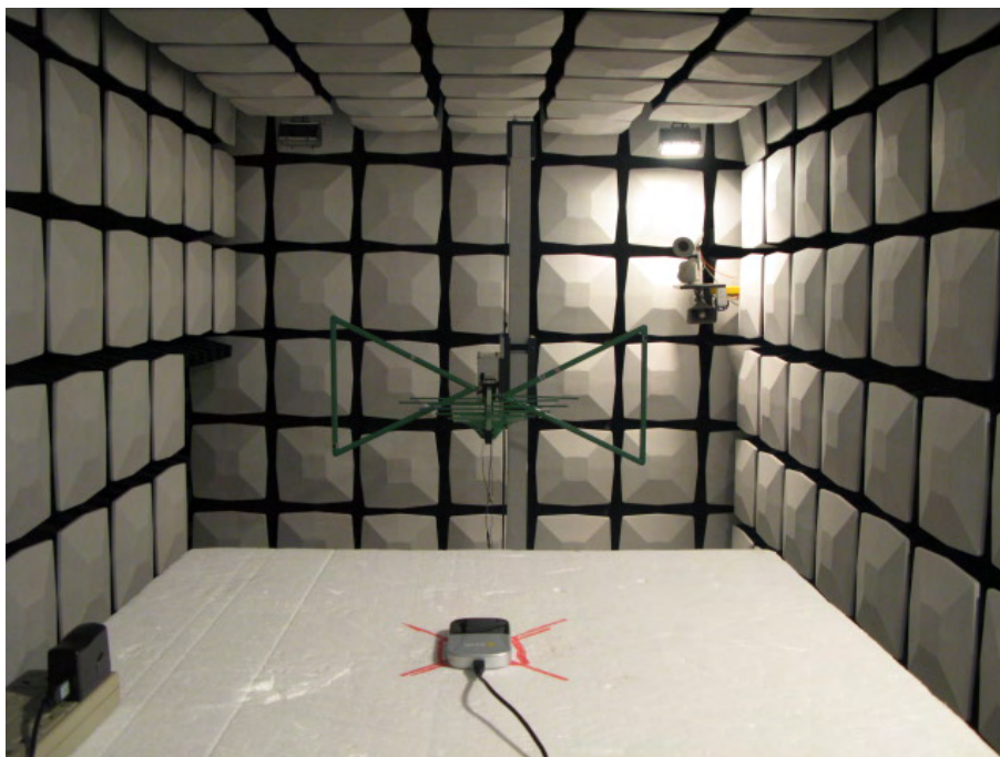
Radiated Spurious Emission (below 2GHz) CDMA
