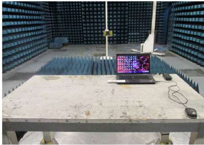
Radiated Emission of 1-18G
