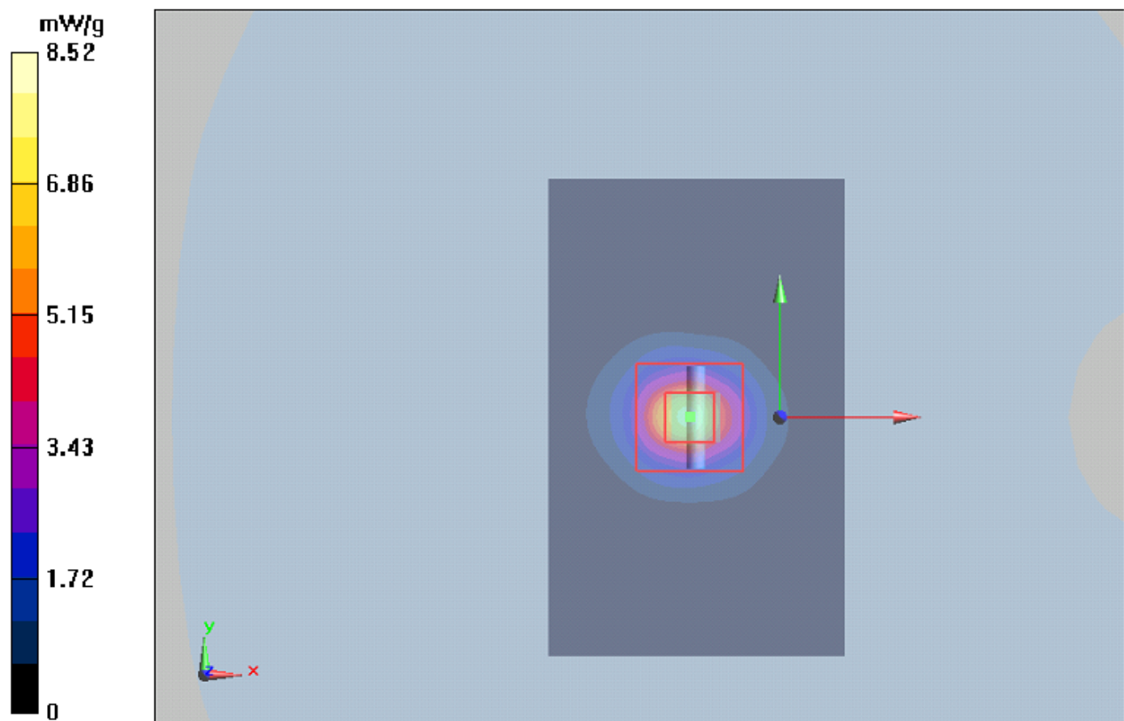
Figure 117 System Performance Check 5800MHz 100mW
