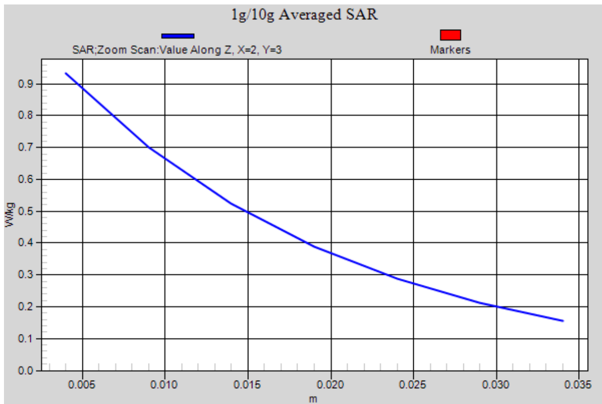
Figure 120 UMTS Band V with Test Position 1 Channel 4132
