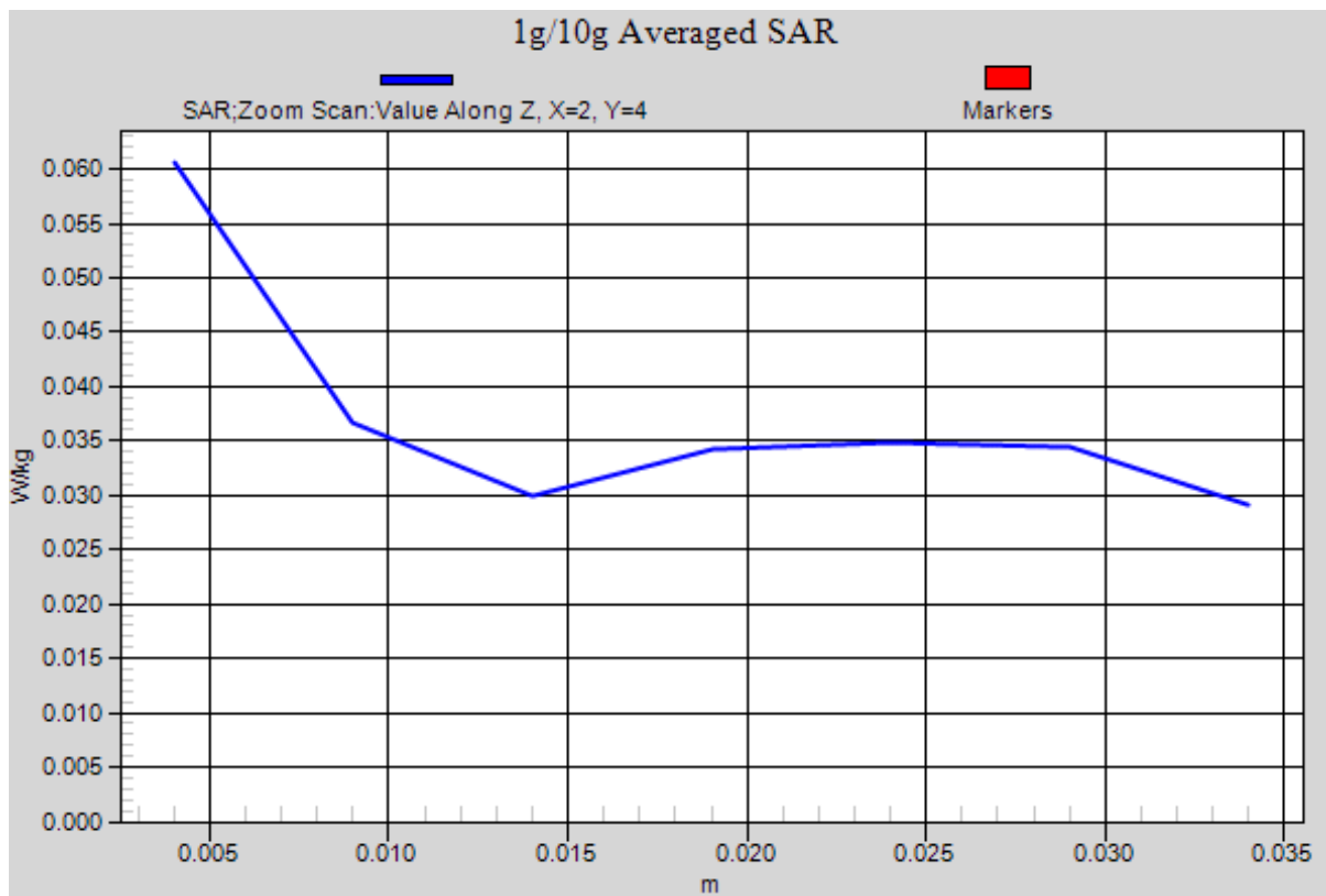
Figure 123 802.11a with Test Position 2 Channel 157
