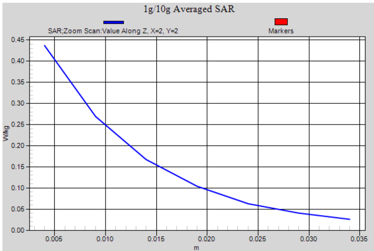
Figure 119 GSM 1900 GPRS (2TXslots) with Test Position 2 Channel 661
