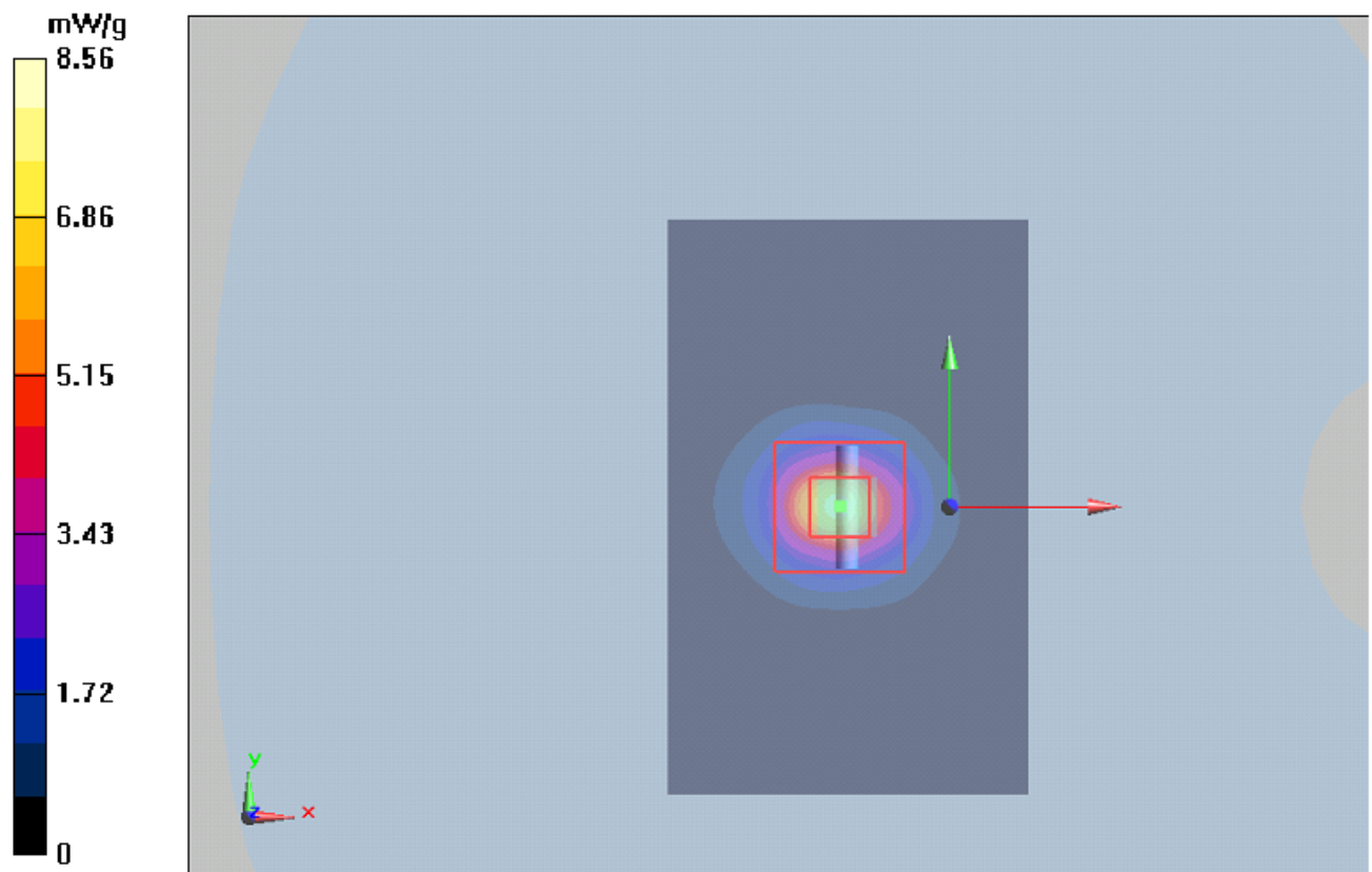
Figure 116 System Performance Check 5200MHz 100mW
