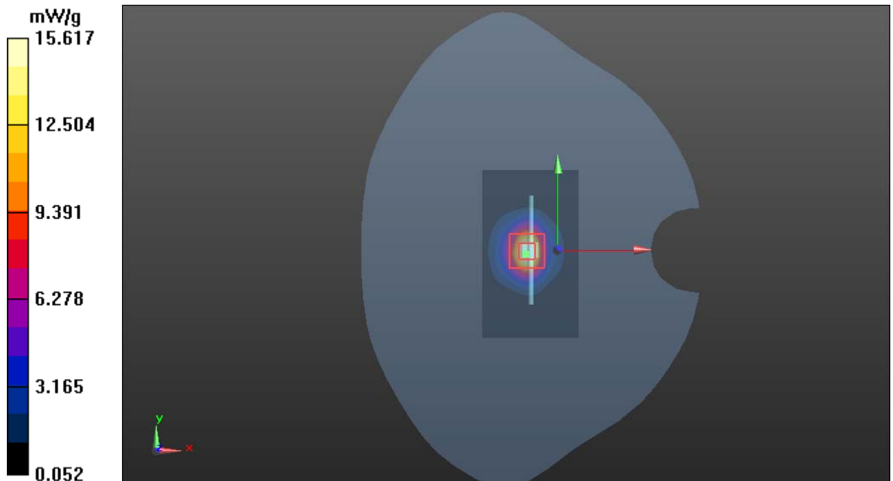
Figure 115 System Performance Check 2600MHz 250mW
