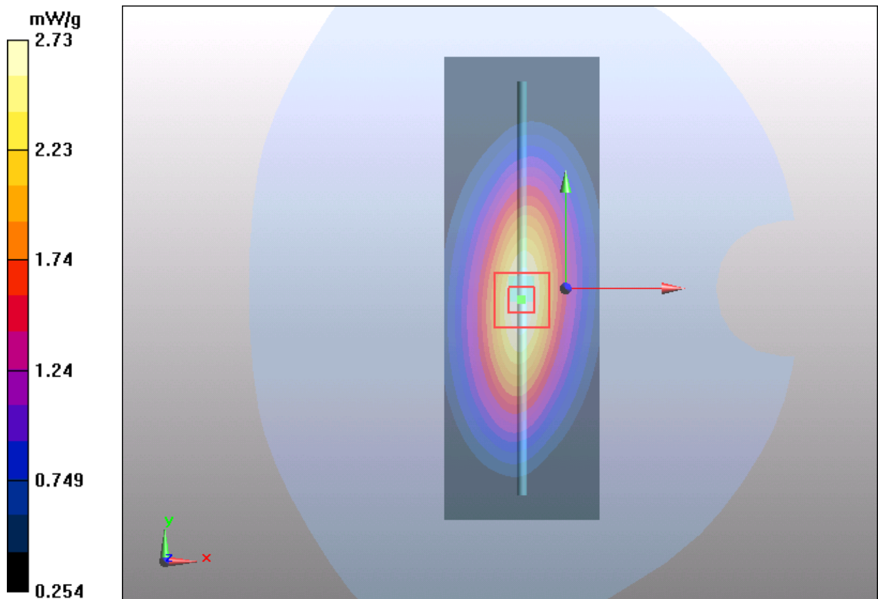
Figure 112 System Performance Check 835MHz 250Mw
