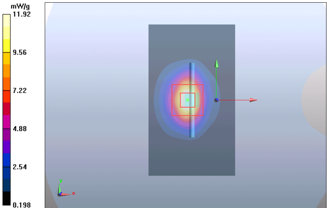
Figure 113 System Performance Check 1900MHz 250mW
