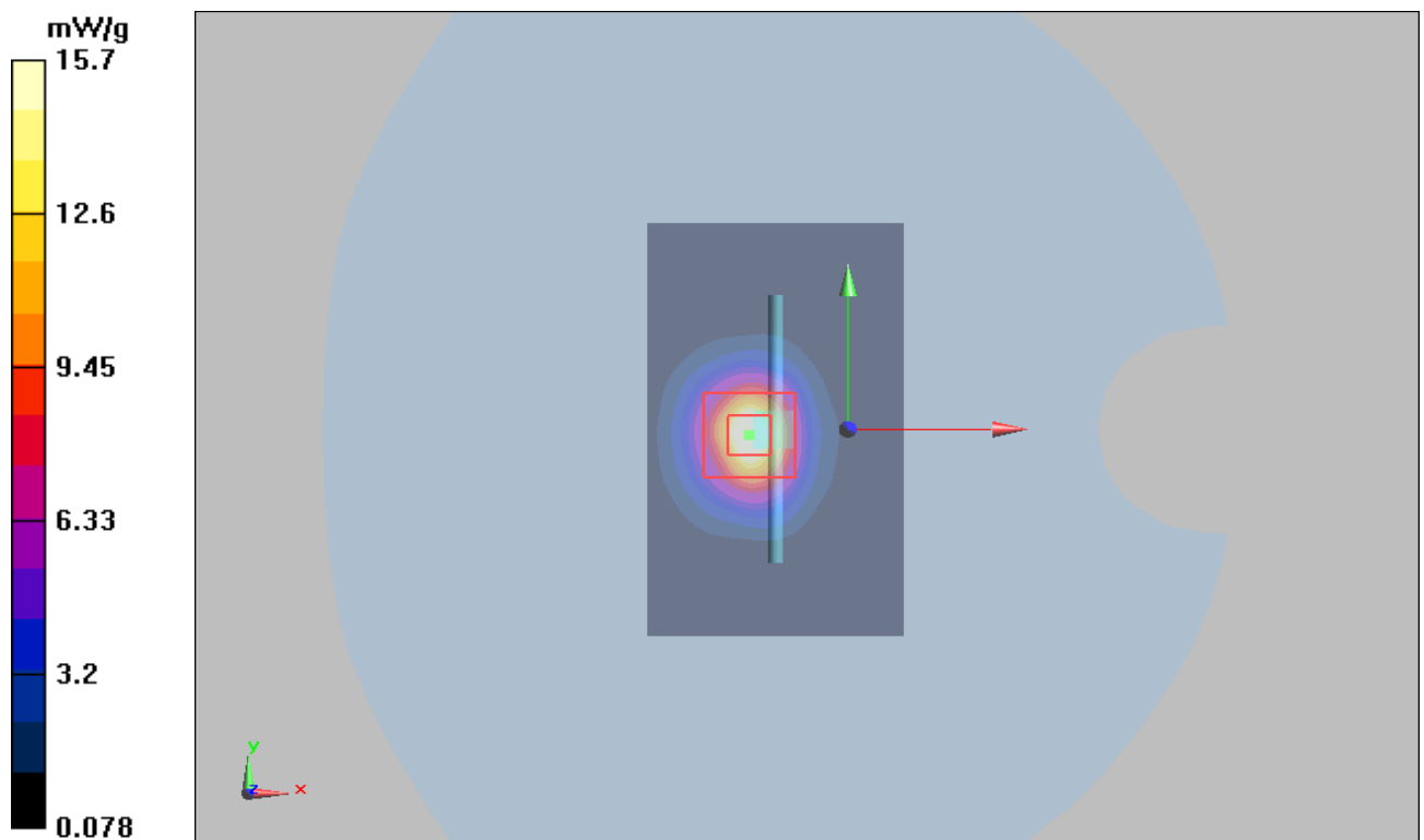
Figure 114 System Performance Check 2450MHz 250mW
