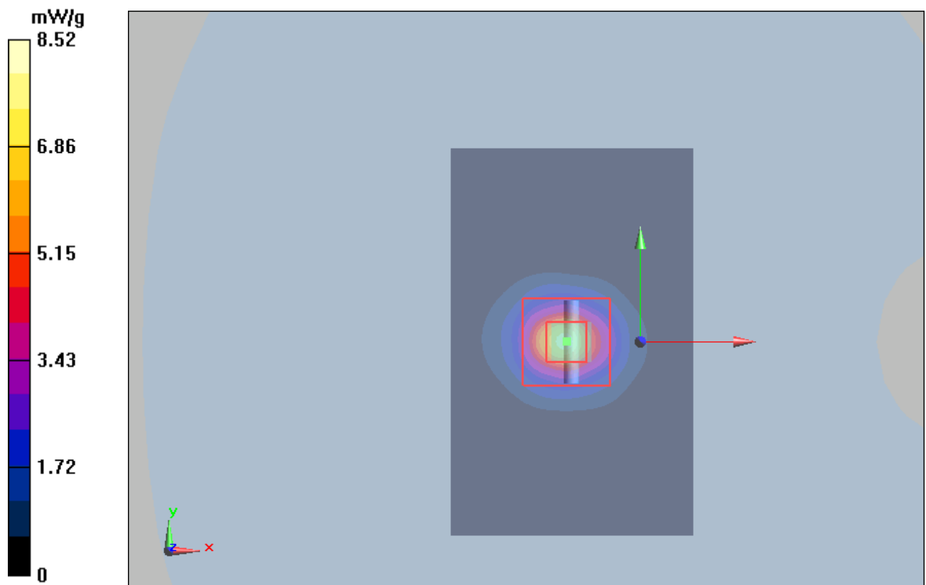
Figure 10 System Performance Check 5200MHz 100mW
