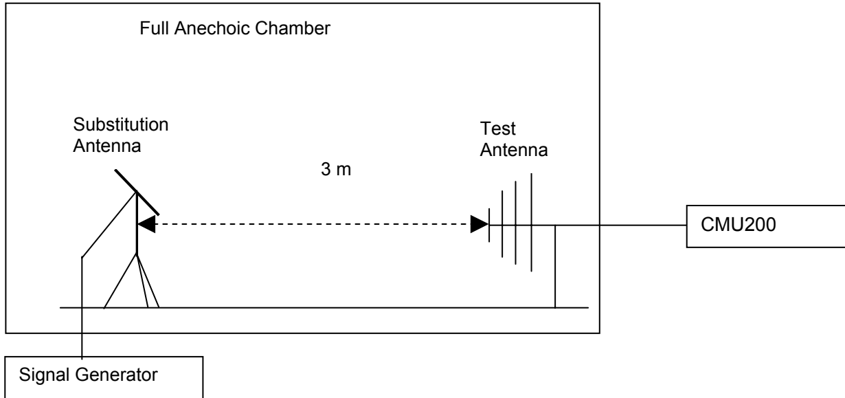
Figure 1. Test Set-up
