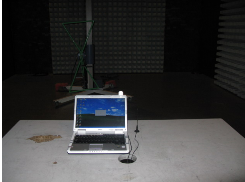
Radiated Disturbance
