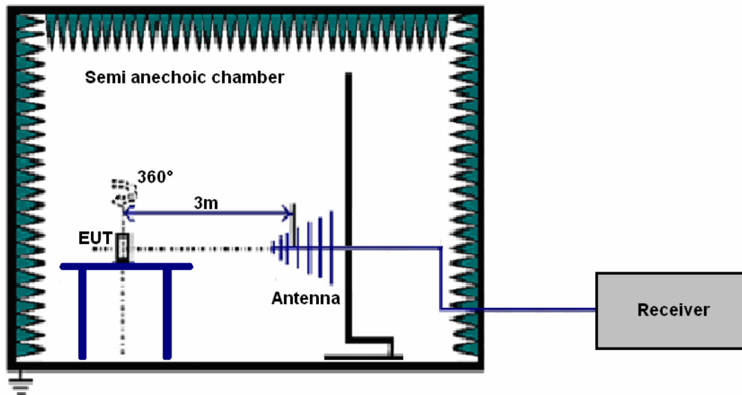
Figure 3. Test set-up
