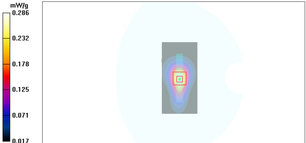
Figure 21 GSM 850 GPRS (4Up) with Lenovo Y-450 Test Position 3 Channel 192
