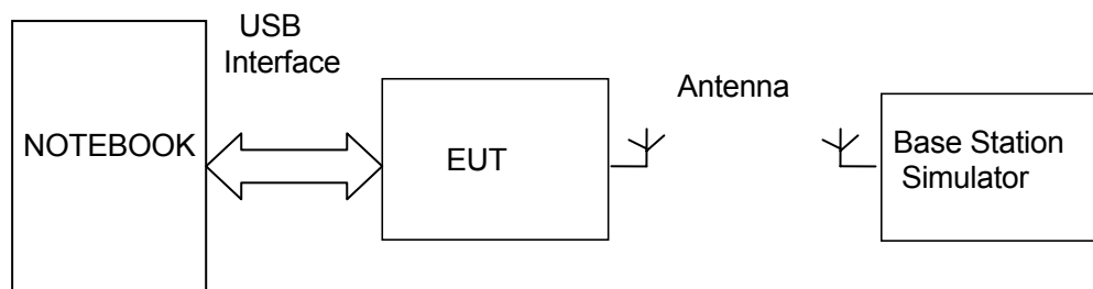
Figure 2. TC1 (TM5-TM8)
