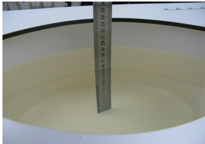
Photo 19: MSL835MHz depth (15.1cm)
