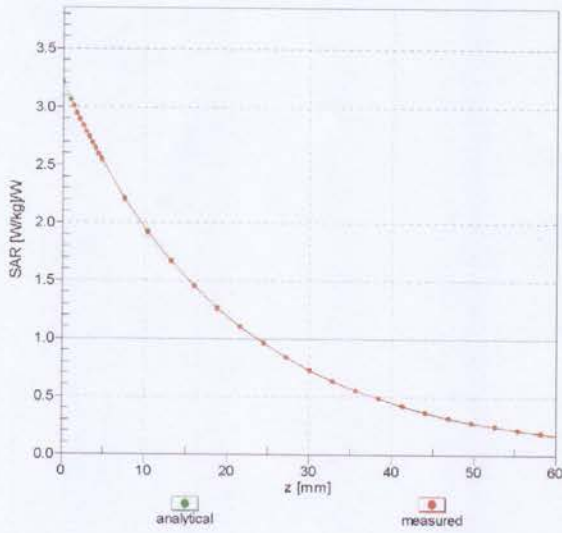
f = 850 MHz, WGLS R9 (H_convF)
