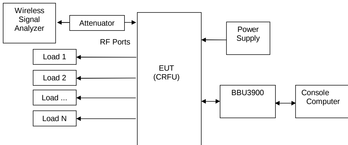
Figure 1. TEST SETUP
