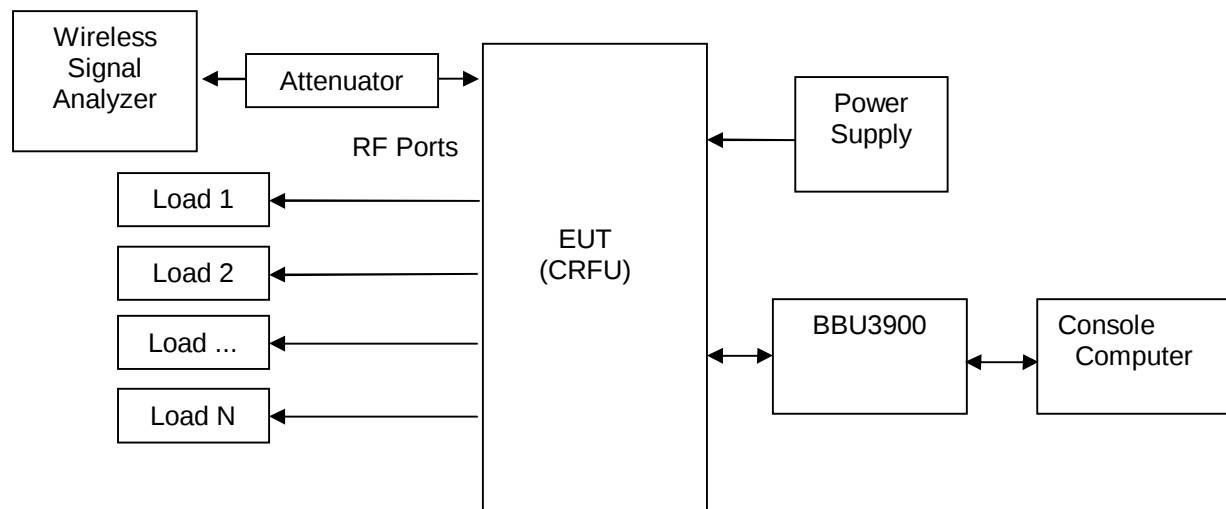
Figure 4. TEST SETUP
