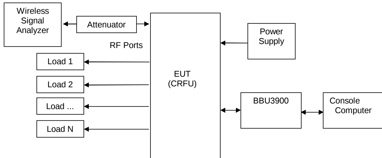
Figure 5. TEST SETUP
