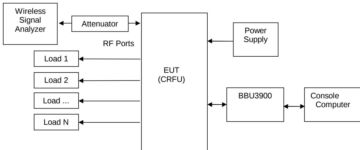
Figure 3. TEST SETUP
