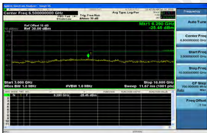
3GHz~10GHz_Band26_3MHz_QPSK_1_0_LowCH26705
