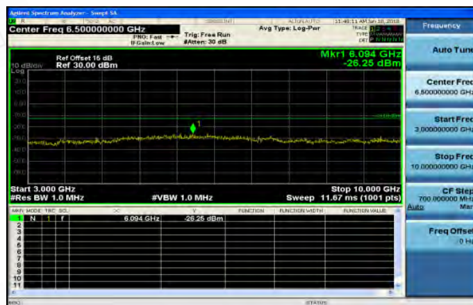
3GHz~10GHz_Band26_3MHz_QPSK_1_0_MidCH26740
