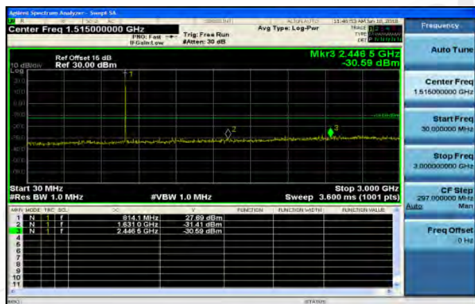
30MHz~3GHz_Band26_3MHz_QPSK_1_0_LowCH26705
