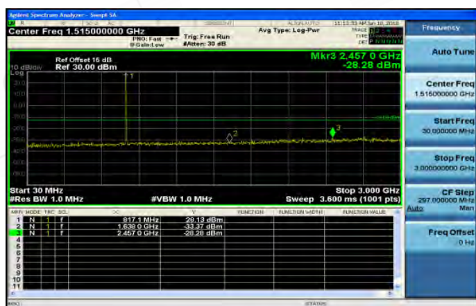
30MHz~3GHz_Band26_5MHz_QPSK_1_0_MidCH26740
