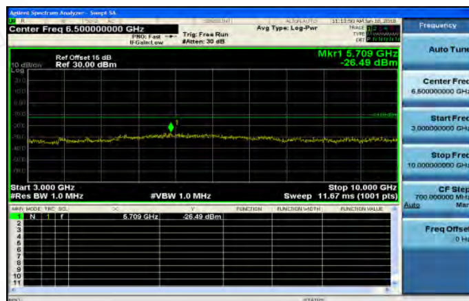
3GHz~10GHz_Band26_5MHz_QPSK_1_0_MidCH26740
