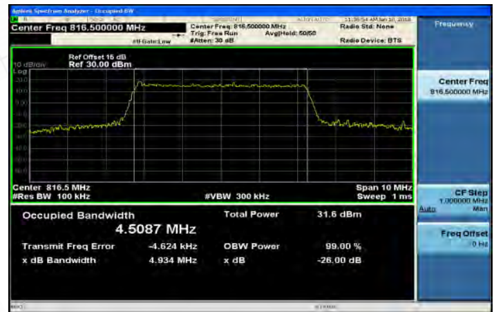
Part 90_Band26_5MHz_16QAM_25_0_MidCH26715
