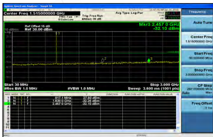
30MHz~3GHz_Band26_3MHz_QPSK_1_0_MidCH26740
