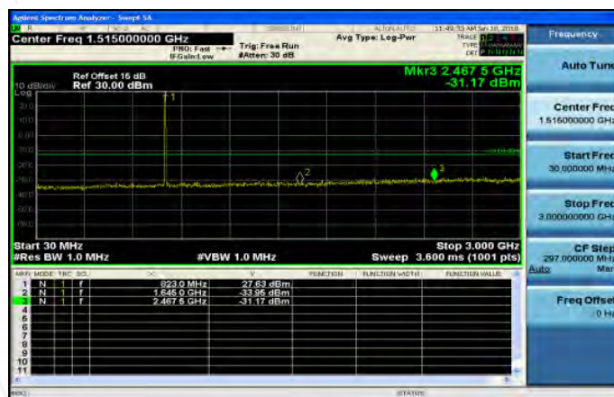
30MHz~3GHz_Band26_3MHz_QPSK_1_0_HighCH26775
