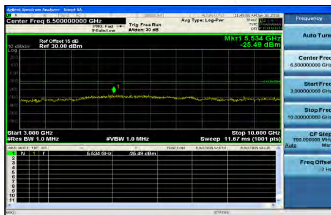
3GHz~10GHz_Band26_3MHz_QPSK_1_0_HighCH26775
