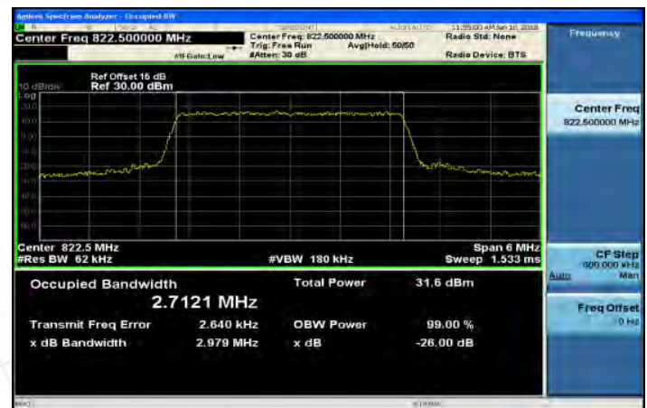
Part 90_Band26_3MHz_QPSK_15_0_HighCH26775
