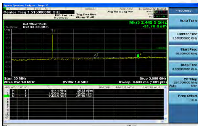
30MHz~3GHz_Band26_5MHz_QPSK_1_0_LowCH26715
