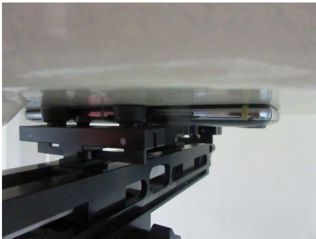
Photo 15: Bottom Side_0mm
