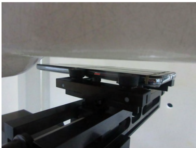
Photo 9: Left Side_10mm
